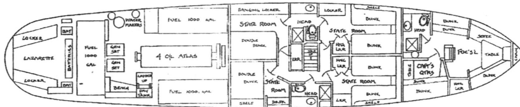
4. Contemporary Sketch and Floor Plan (1988), Westward
