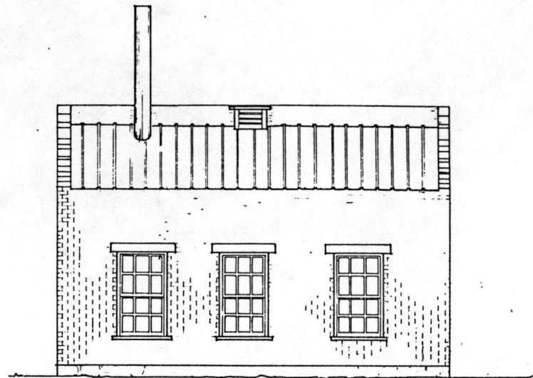
EAST ELEVATION
