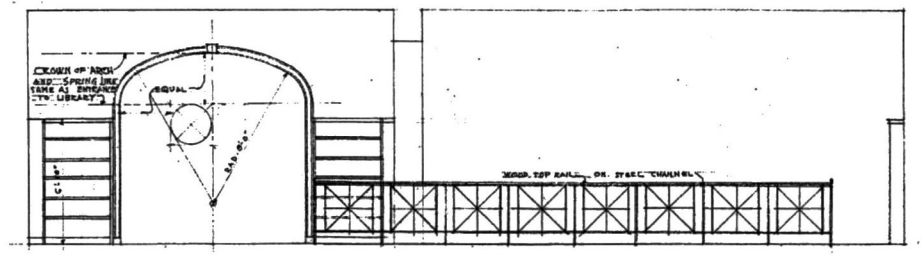
ELEVATION OF EAST WALL WEST WALL SIMILAR LIBRARY STEEL RAILING COMPLETE IS NOT IN CONTRACT
