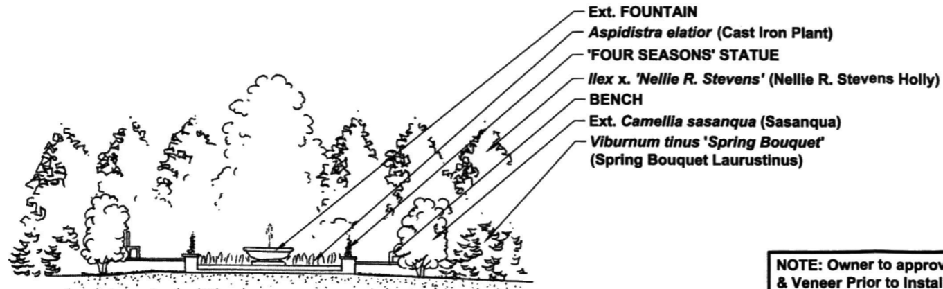
A FOUNTAIN L-1.02 NTS
