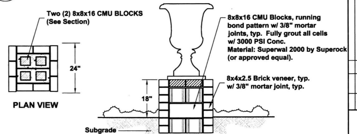
D BRICK PLANTING BED EDGING, TYP. L-1.02 NTS
