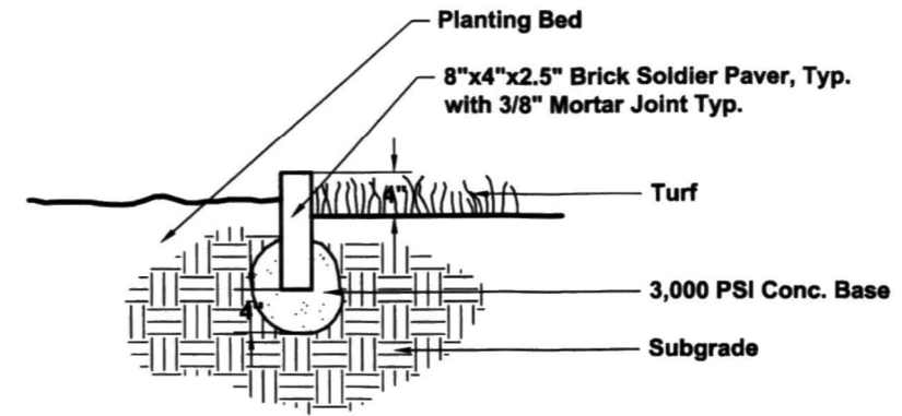
D BRICK PLANTING BED EDGING, TYP. L-1.02 NTS
