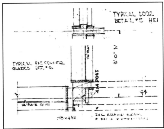
Figure 7: 1948 Plan detail at corner showing expressed verticals
