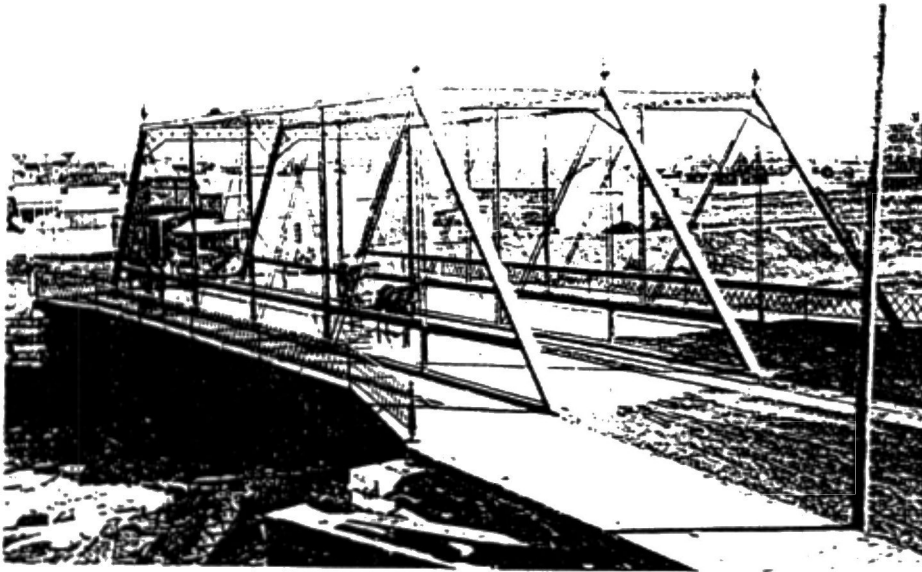
Steel Truss Bridge at Las Vegas. This steel truss bridge was built over the Gallinas River about 1886 and was replaced in 1909 by the existing concrete arch bridge (No 1549). (Photograph Courtesy of the Museum of New Mexico. Negative No. 56291)
