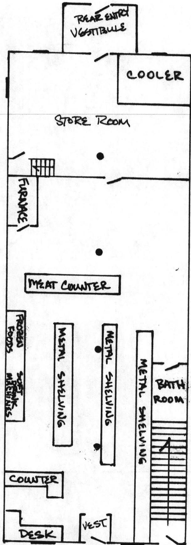
FIRST FLOOR
