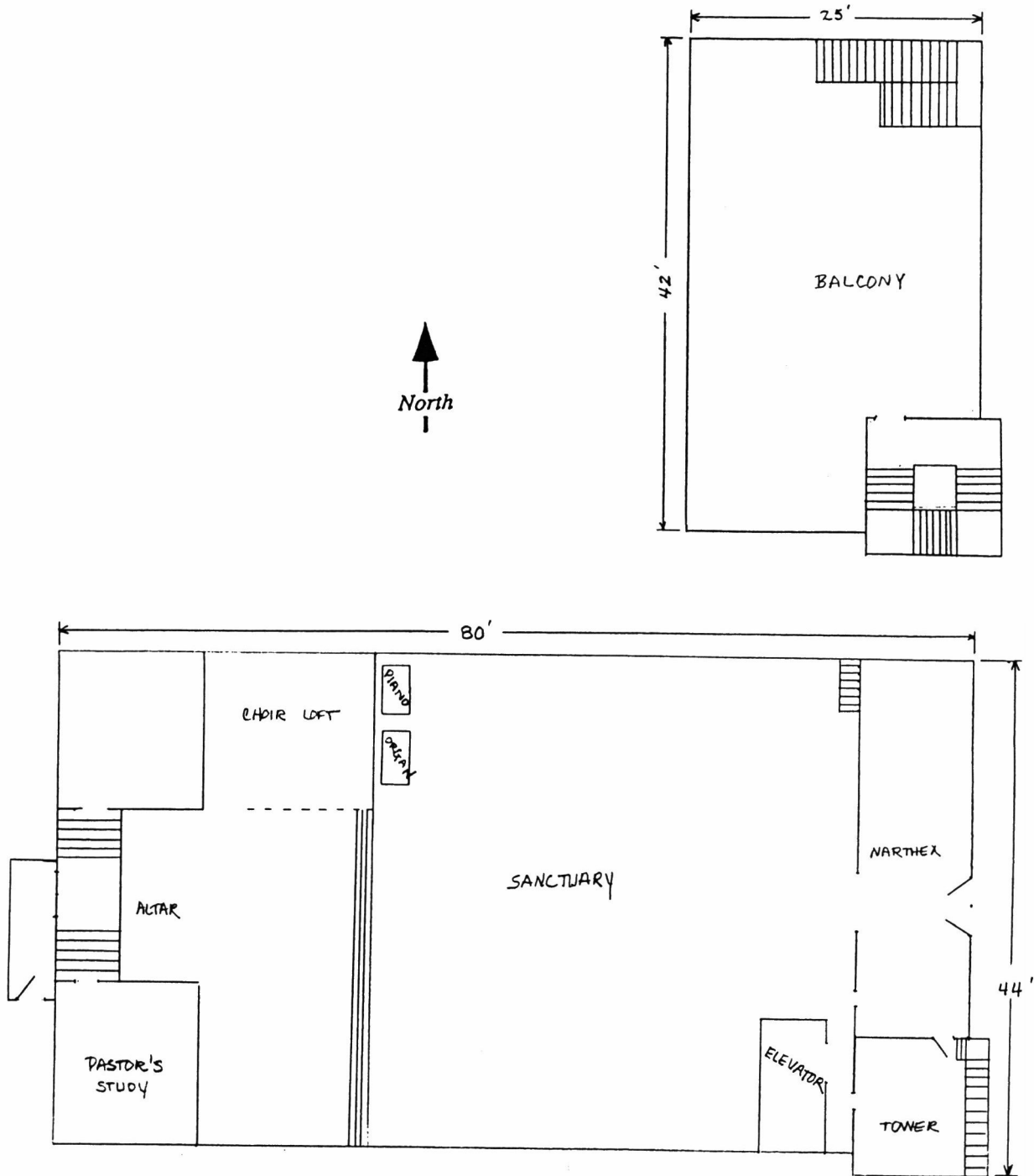
Floor plan of first floor and balcony of church.
