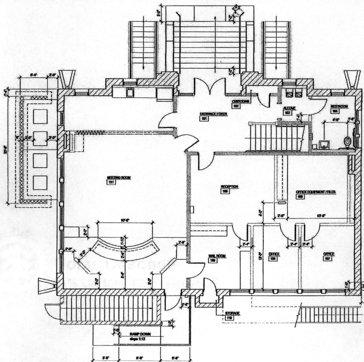
FIRST FLOOR REFERENCE / DIMENSION PLAN SCALE: 1/4" = 1'-0"
