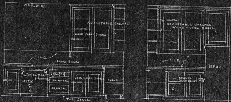
DETAIL OF KITCHEN CABINETS SCALE 1/2" = 1'-0"
