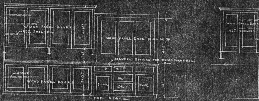
DETAIL OF CABINETS FOR SUNDAY SCHOOL KITCHEN SCALE 1/2" = 1'-0"
