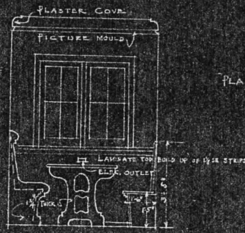
DETAIL OF DINETTE SHOWING SEAT & TABLE SCALE 1/2" = 1'-0"
