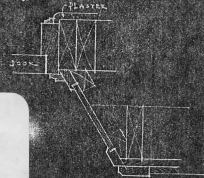
SECTION THRU MAIN ENTRANCE DOOR SCALE 3/4" = 1'-0"
