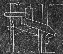
SECTION AT SILL WINDOW DETAIL GALV. IRON SCALE 3/4" = 1'-0"
