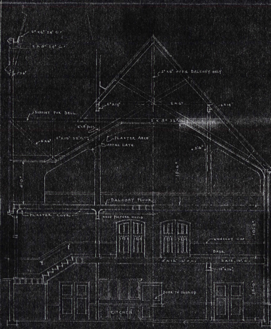
CROSS SECTION ON LINE 'A-A'
