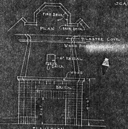
DETAIL OF LIVING ROOM FIRE PLACE
