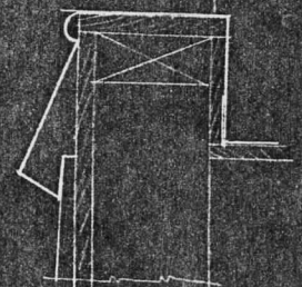
DETAIL OF WALL COPING WEST ELEVATION SCALE 3/4" = 1'-0"
