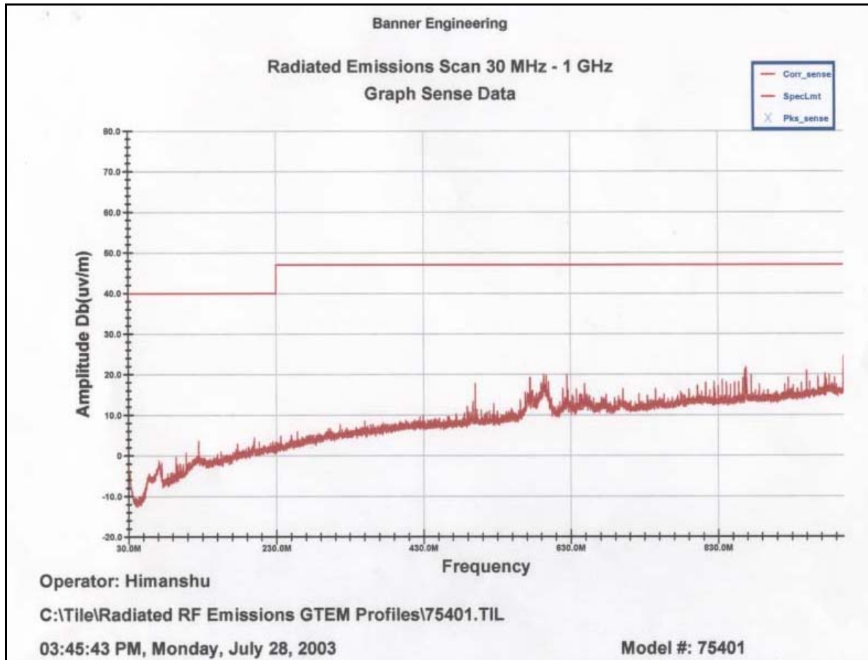
Figure 1.1: LH75401-10/11 Test Results
