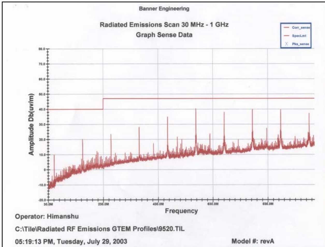
Figure 1.1: LH79520-10 Test Results
