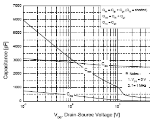
Fig.5 Capacitance Characteristics
