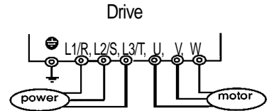
Fig. 3-1-1 Drive connection
