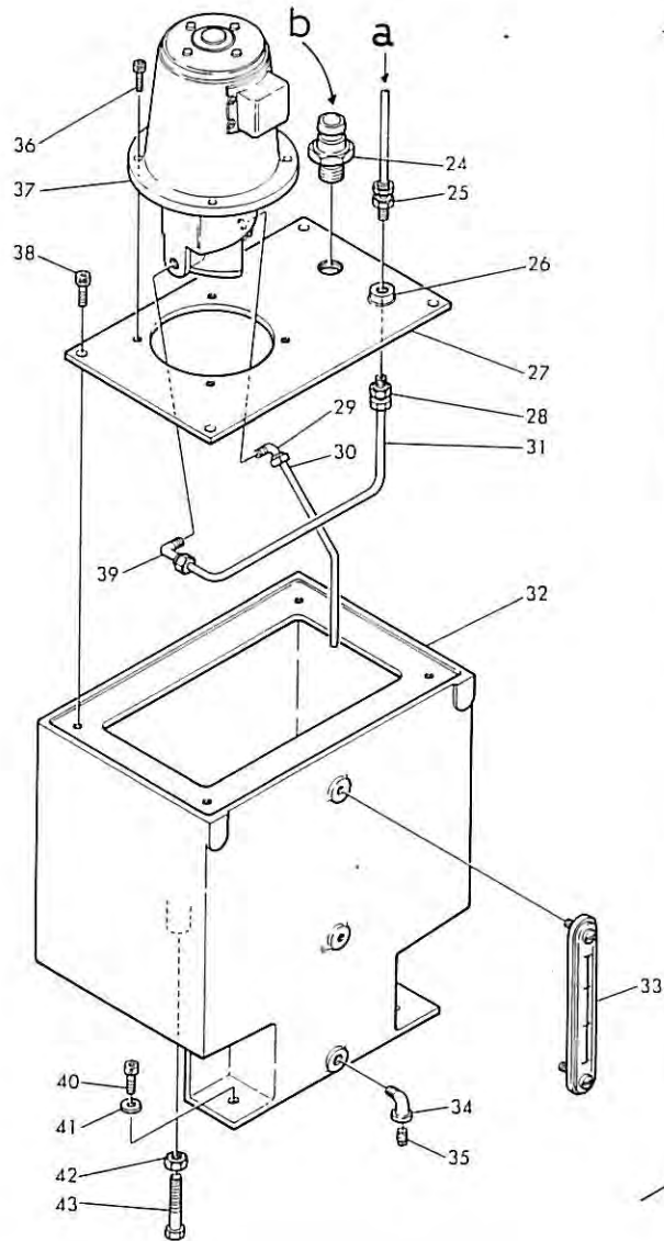
TANK Ass'y
