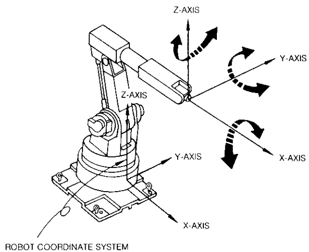
ROBOT COORDINATE SYSTEM
