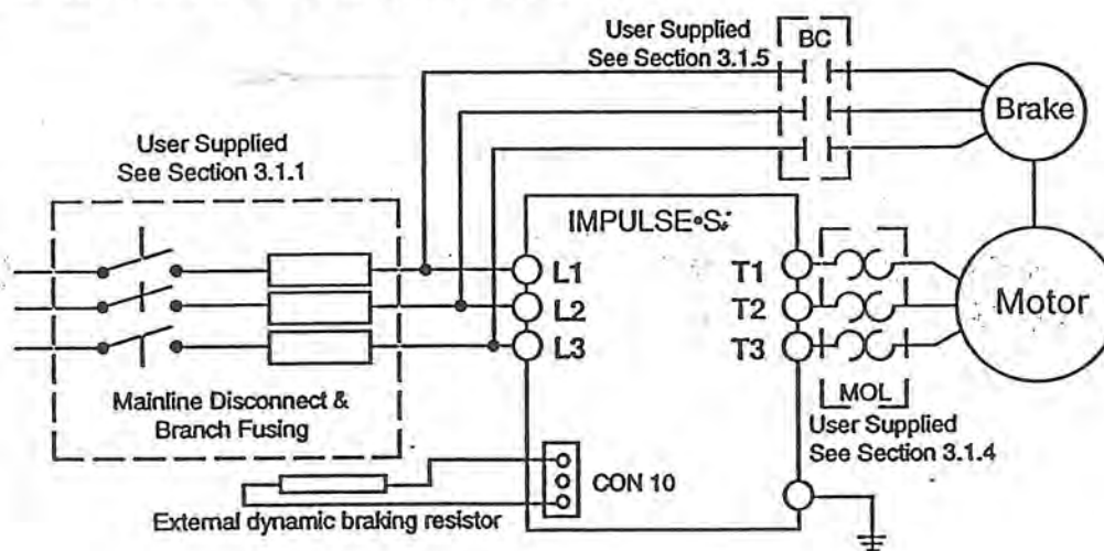
IMPULSE•S ® used with three-phase motor brake
