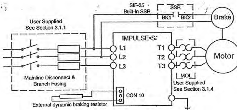
IMPULSE•S ® used with single-phase brake coils
