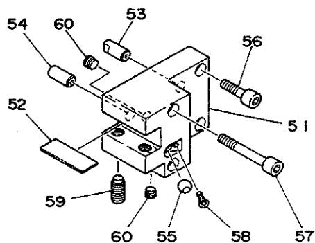
#6L78 4500 TURNING TOOL HOLDER
