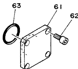
#6M78 0900 COVER
