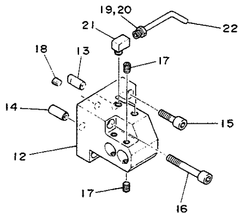
#6M78 4200 DOUBLE PLAIN HEAD B
