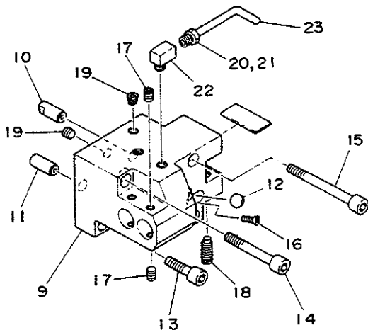
DOUBLE &amp; TURNING HOLDER R
