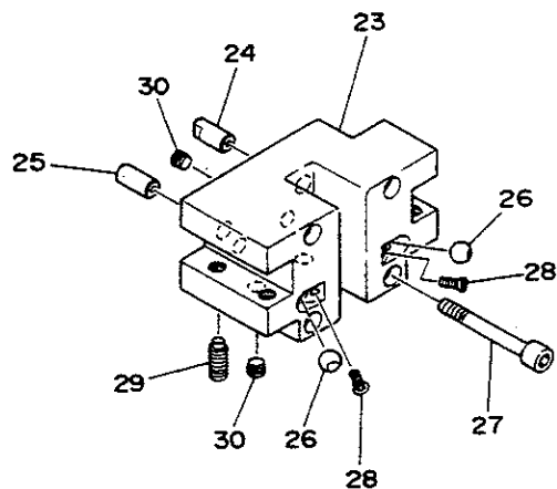
#6L78 430A DOUBLE TURNING HOLDER A
