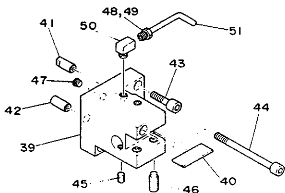
#6M78 5000 TURNING & PLAIN HOLDER
