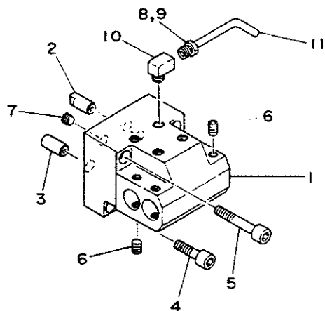
#6M78 410A DOUBLE PLAIN HEAD A
