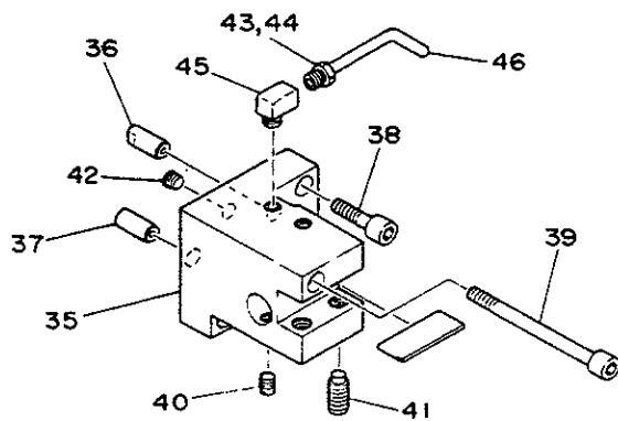
#6M78 500A TURNING & PLAIN HOLDER
