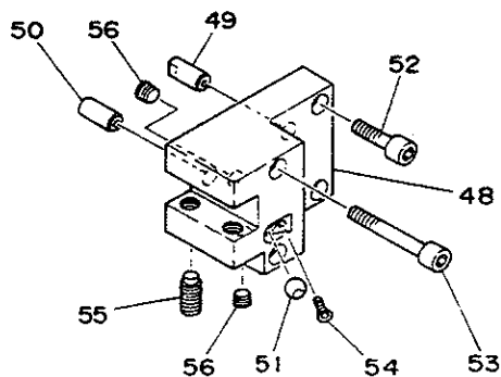
#6L78 450A TURNING TOOL HOLDER
