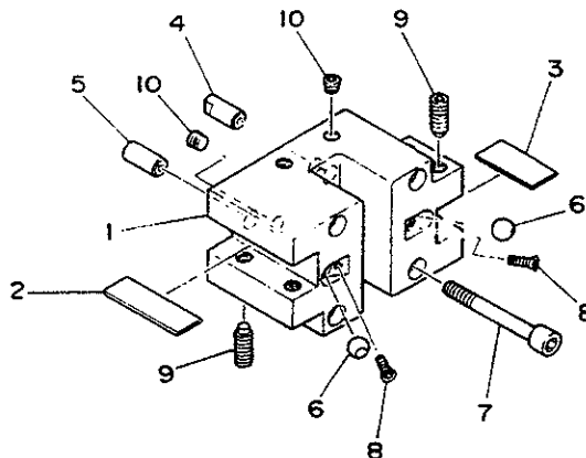
#6L78 4700 DOUBLE TURNING HOLDER B
