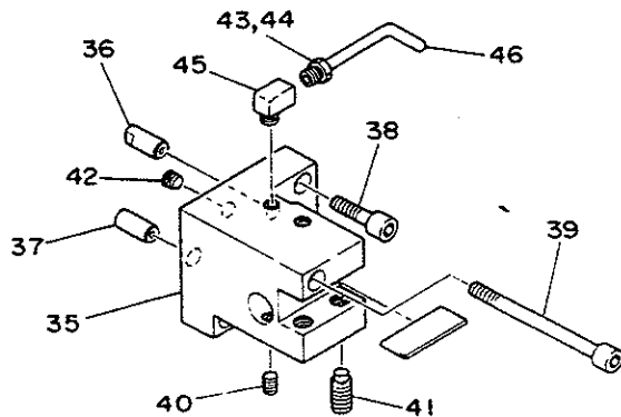
TURNING &amp; PLAIN HOLDER
