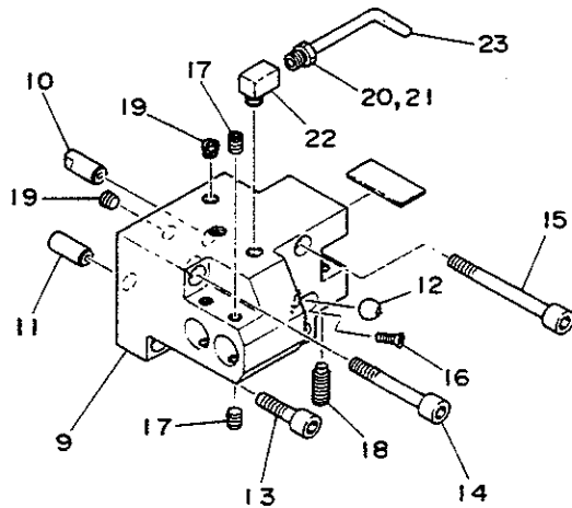
#6M78 500A TURNING & PLAIN HOLDER
