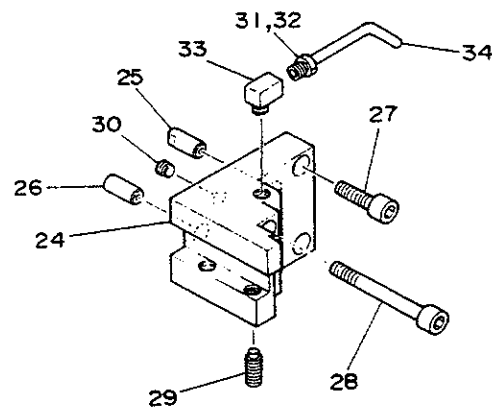
CUT-OFF TOOL HOLDER
