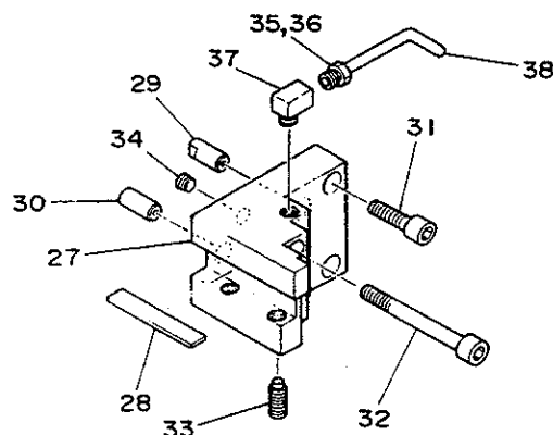
#6M78 4900 CUT-OFF TOOL HOLDER
