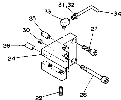
#6M78 490A CUT-OFF TOOL HOLDER
