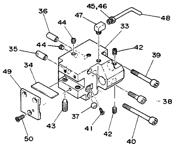
#6M78 4400 DOUBLE & TURNING HOLDER F
