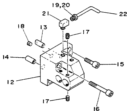
#6M78 420A DOUBLE PLAIN HEAD B
