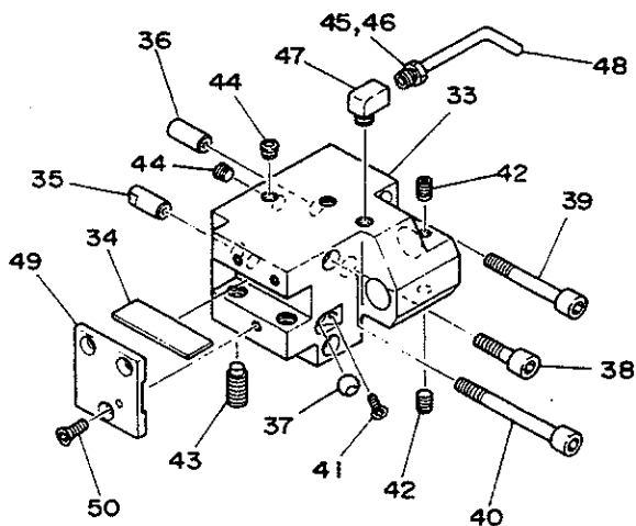
#6M78 4400 DOUBLE & TURNING HOLDER F
