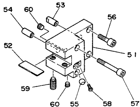
#6L78 4500 TURNING TOOL HOLDER
