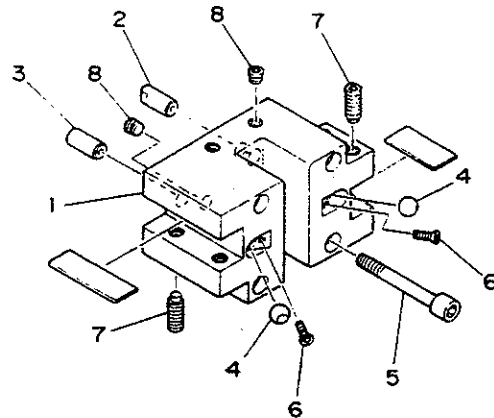
#6L78 470A DOUBLE TURNING HOLDER B
