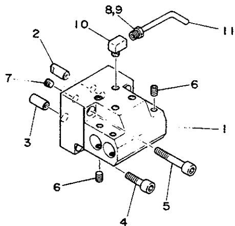
#6M78 4100 DOUBLE PLAIN HEAD A
