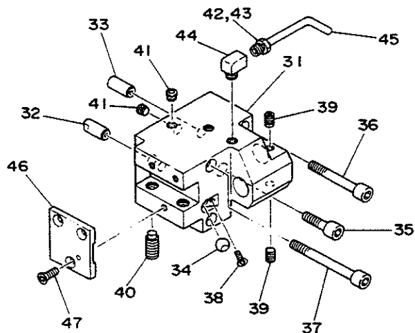
#6M78 440A DOUBLE & TURNING HOLDER F
