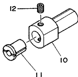
#5E78 1400 DRILL HOLDER
