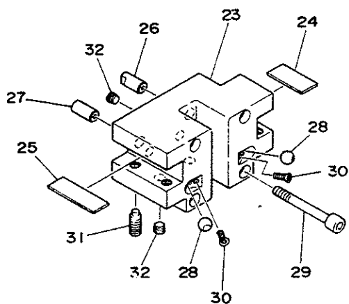
#6L78 4300 DOUBLE TURNING HOLDER A
