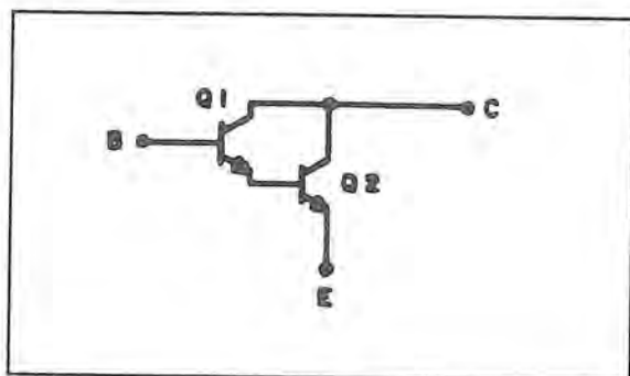
Figure 9-12. Darlington Transistor - Schematic Diagrams.
