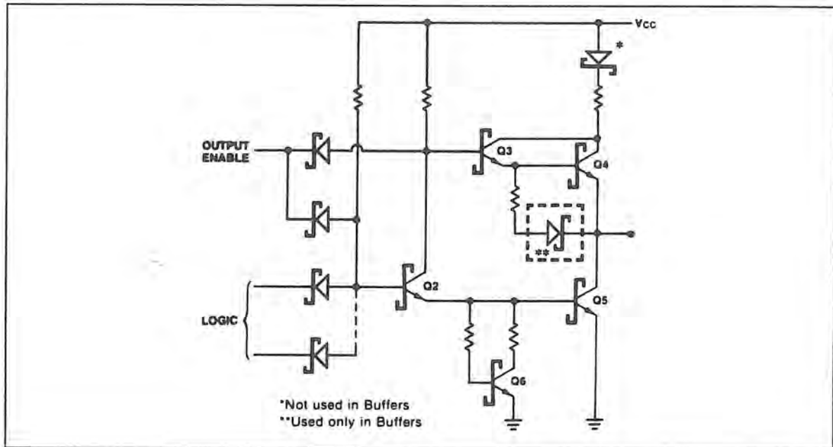
Figure 12-38. Typical Tri-State Output Control.
