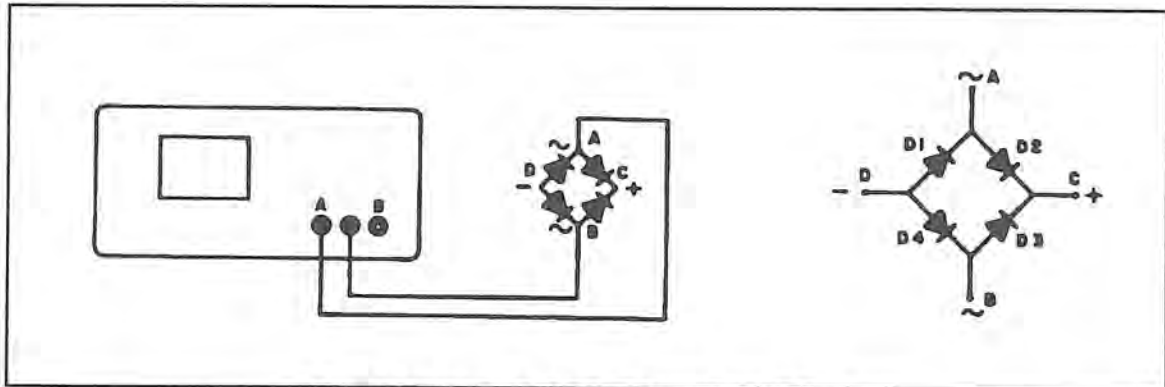
Figure 8-11. Rectifier Bridge Test Connections - AC Input.
