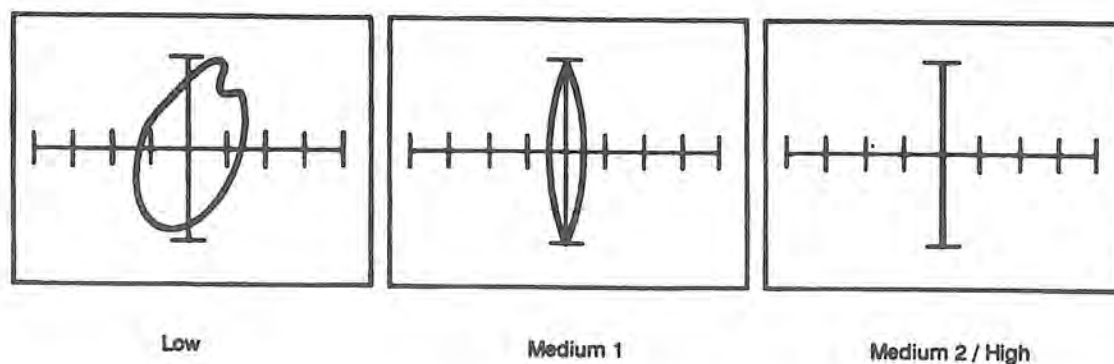
Figure 13-9. Signatures of a Defective Capacitor.
