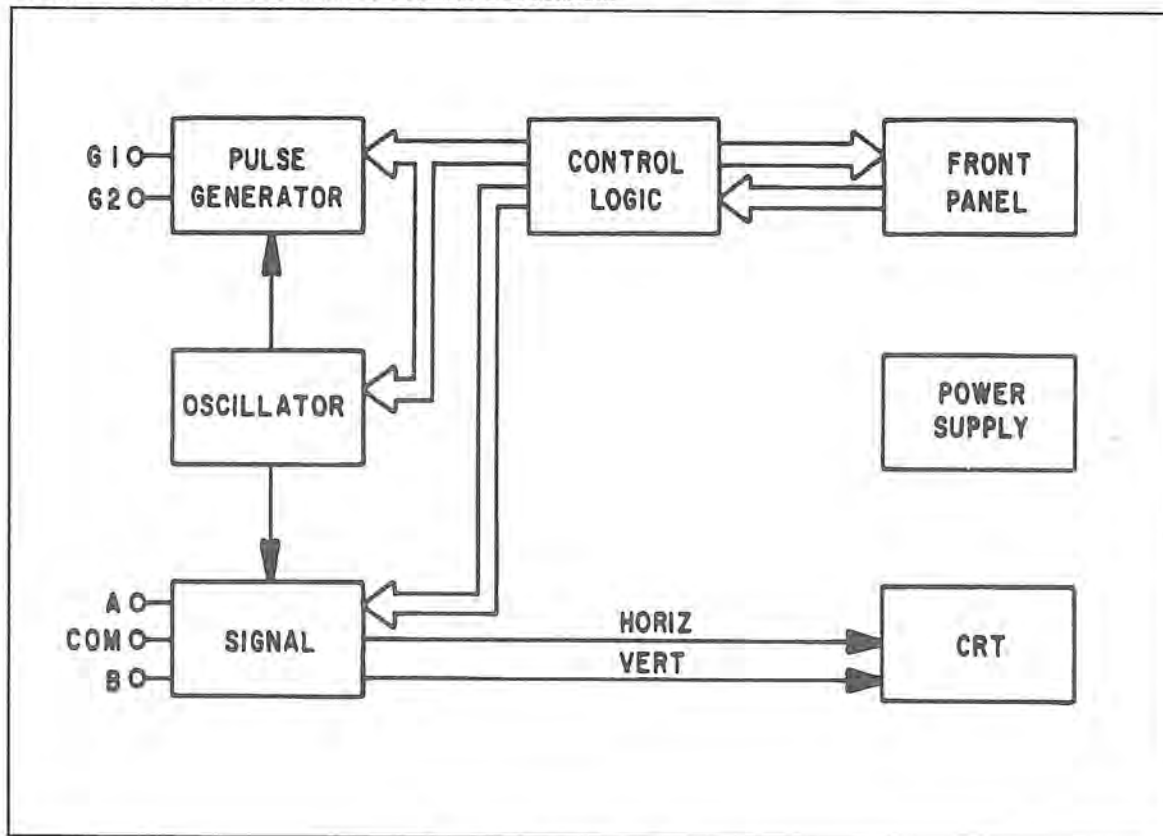
Figure 3-1. 2000 Block Diagram.
