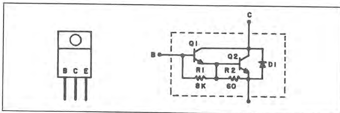
Figure 9-13. The TIP112 Darlington Transistor.
