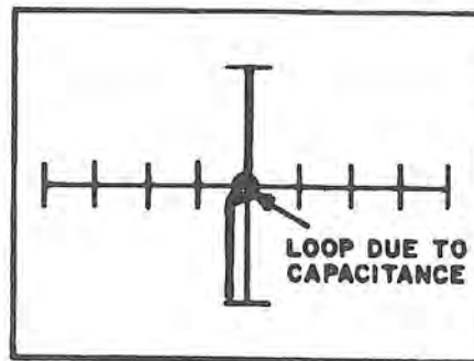
Figure 8-25. Signature of a PN2222 B-E Junction in High Range at 2000 Hz.
