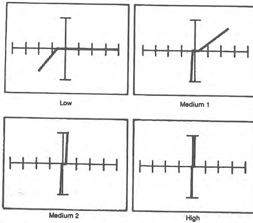
Figure 12-37. Signatures Between the V_{cc} Pin and Ground Pin of a 74LS32 at 60 Hz.
