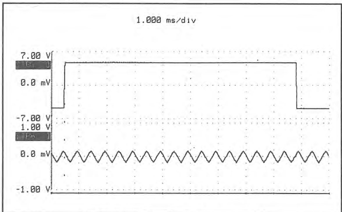
Figure 4-15. Signal PCB Waveforms: TP1 & TP6 - Settings: 2000 Hz.
