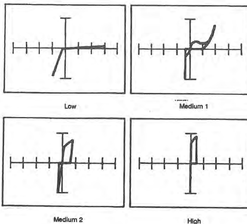
Figure 12-45. Signatures Between an Output Pin and V_{ss}-V_{dd} of a 4011B at 60 Hz.
