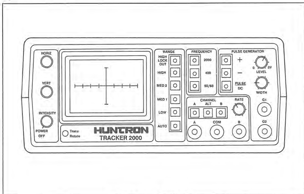
Figure 1-1. Huntron Tracker 2000.
