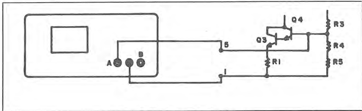
Figure 12-26. Test Circuit of an LM555 Pin 5 and Pin 1.
