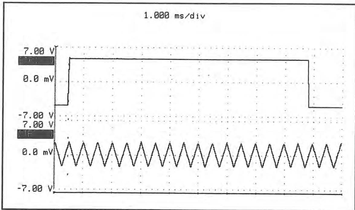
Figure 4-12. Signal PCB Waveforms: TP1 & TP5 - Settings: 2000 Hz.
