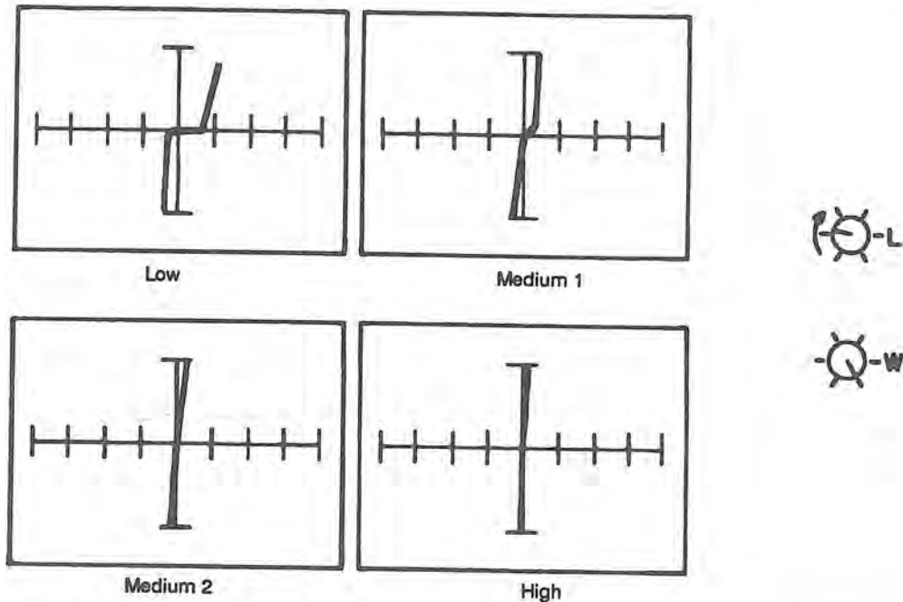
Figure 10-12. MT1-MT2 Signatures of a 2N6070 Triac with Gate Connected to Pulse Generator at 60 Hz.
