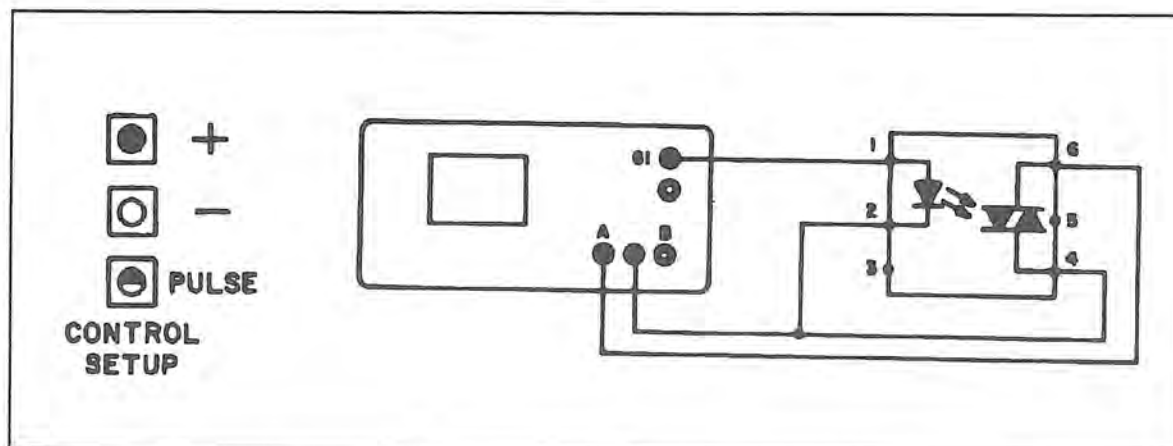
Figure 10-38. Test Circuit for a MOC3010 Triac with Pulse Generator.
