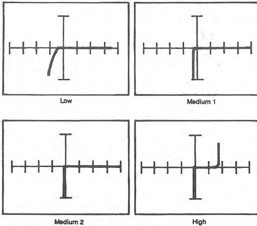
Figure 12-33. Signatures Between an Output Pin and the Ground Pin of a 7410 at 60 Hz.
