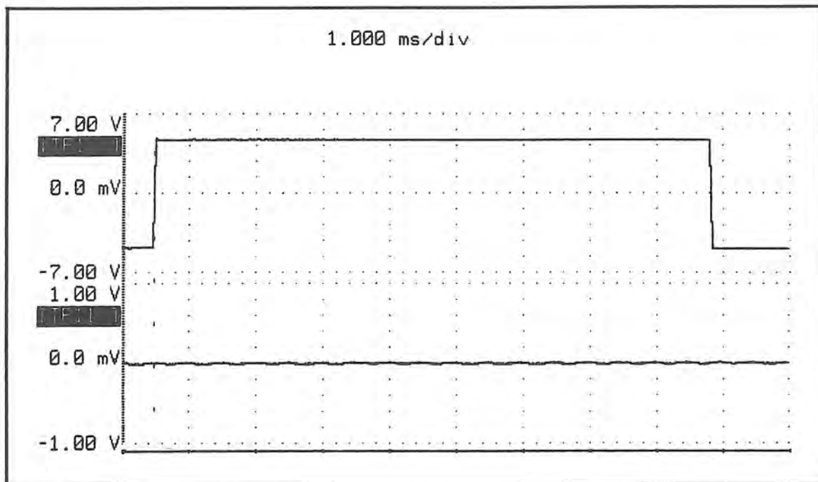
Figure 4-20. Signal PCB Waveforms: TP1 & TP11 - Settings: 2000 Hz, open circuit, LOW range.
