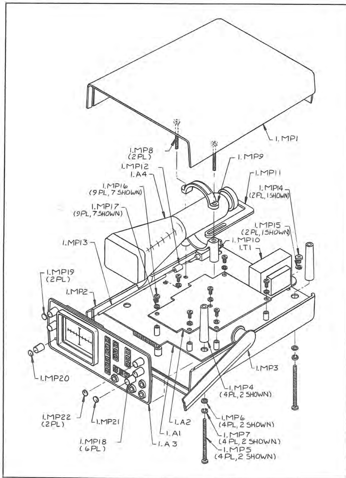
Figure 5-1. Final Assembly.
