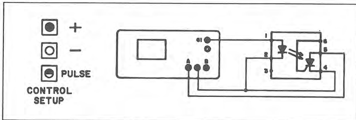
Figure 10-33. Test Circuit for an H11C3 with Pulse Generator.
