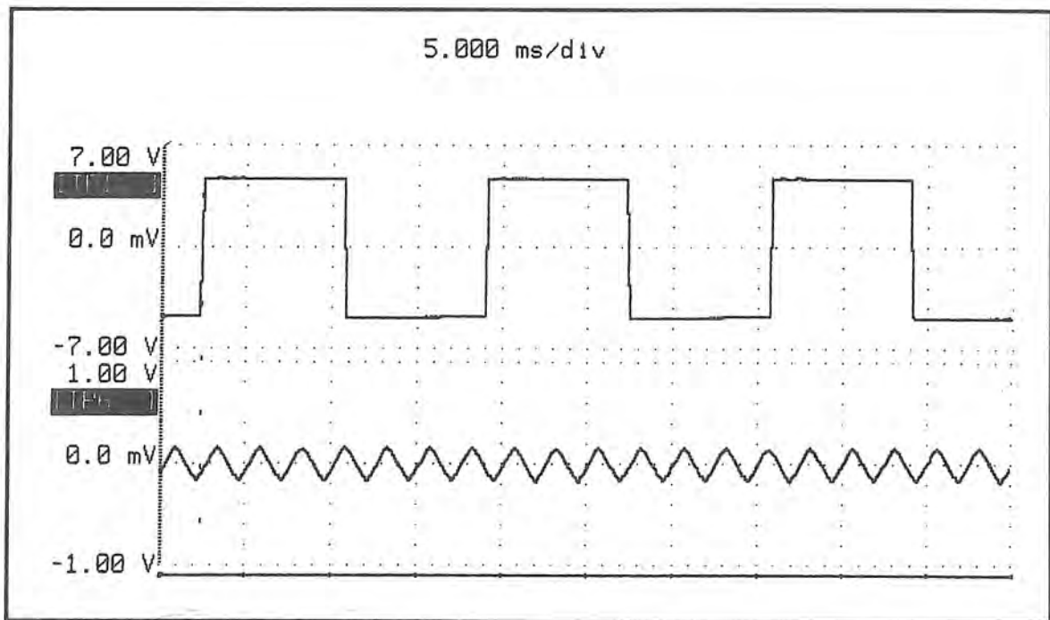
Figure 4-14. Signal PCB Waveforms: TP1 & TP6 - Settings: 400 Hz.
