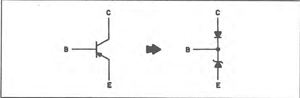
Figure 9-7. Equivalent Circuit of a PNP Transistor.
