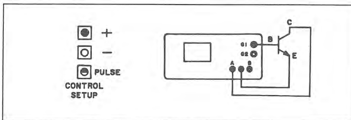
Figure 10-13a. NPN Transistor Test Circuit Using Pulse Generator.
