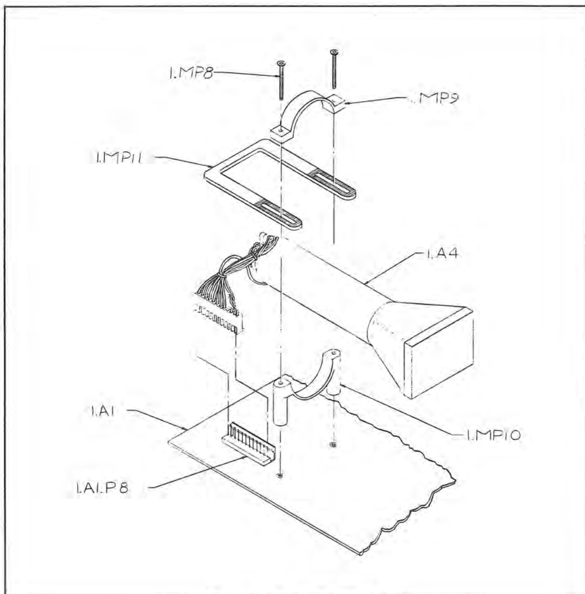
Figure 4-2. CRT Assembly Removal.
