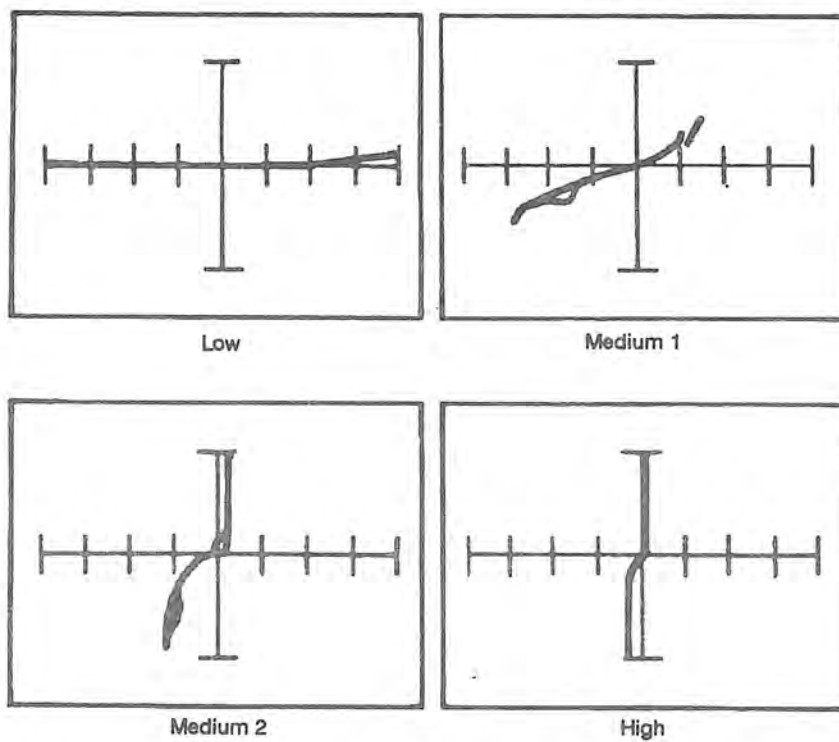
Figure 12-61. Signatures Between the V_{dd} Pin and the V_{ss} JPin of a 2708JL at 60 Hz.
