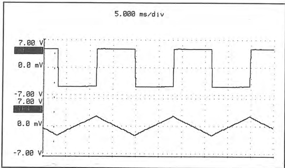
Figure 4-10. Signal PCB Waveforms: TP1 & TP4 - Settings: n.a.
