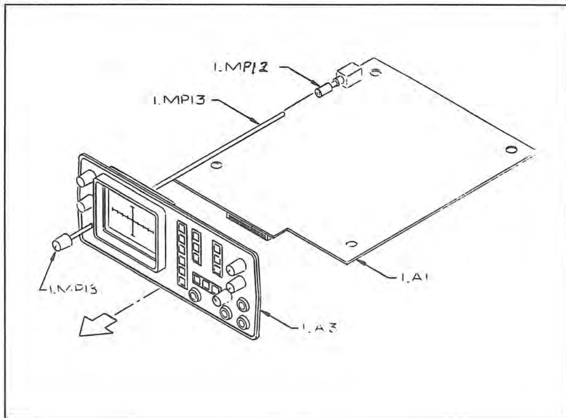
Figure 4-6. Front Control Assembly Removal.
