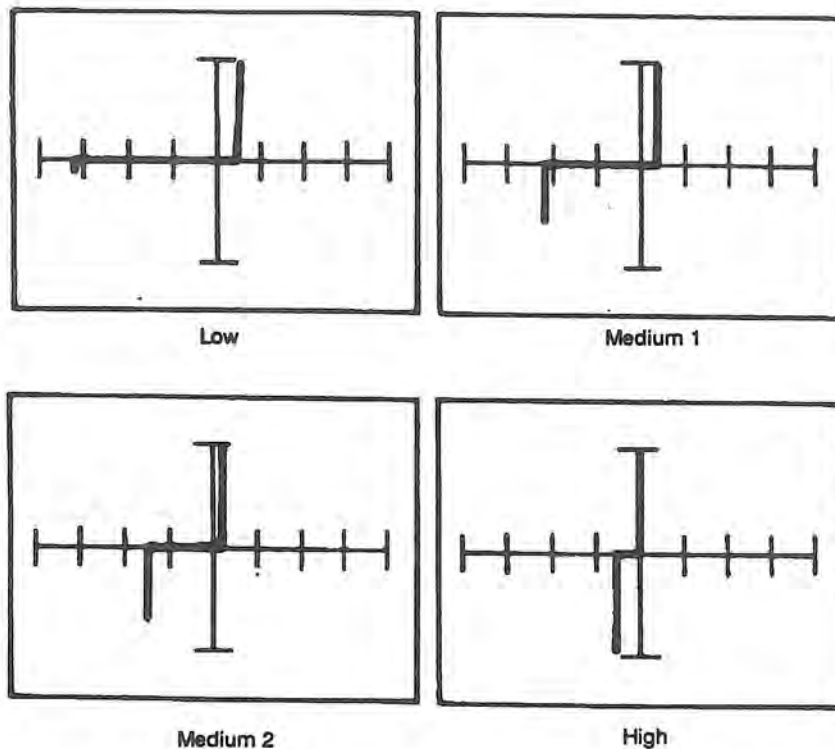
Figure 9-4. Signatures of an NPN Transistor (2N3904) at 60 Hz Base with Emitter as Common.
