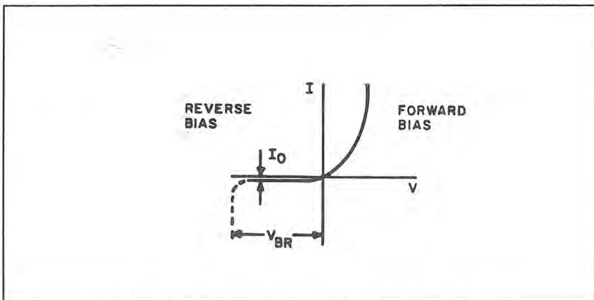
Figure 8-4. The Volt-Ampere Characteristic of a Semiconductor Diode.
