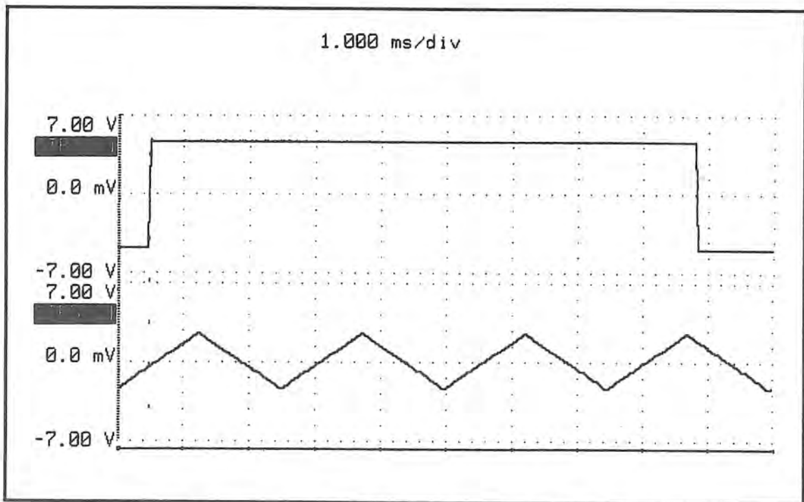
Figure 4-11. Signal PCB Waveforms: TP1 & TP5 - Settings: 400 Hz.
