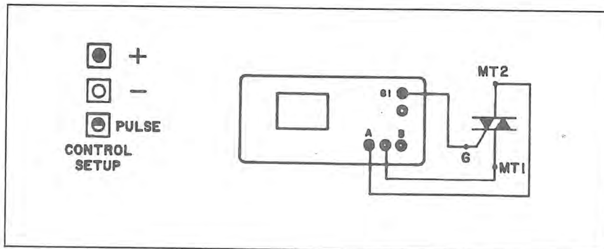
Figure 10-11. Triac Test Circuit Using Pulse Generator.
