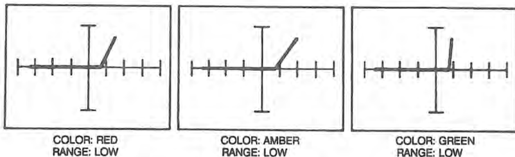
Figure 8-19. LED Signatures.
