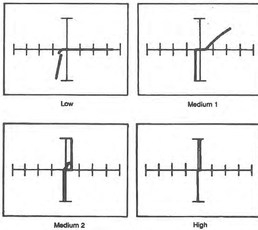
Figure 12-9. Signatures Between Pin 1 (Output) and Pin 2 (V-) of an LM1458 at 60 Hz.
