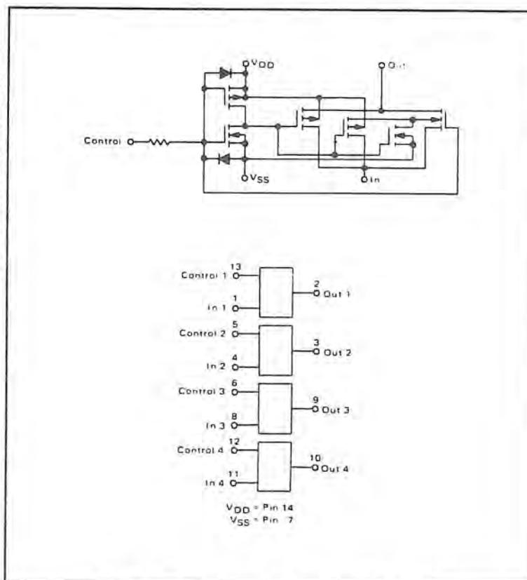
Figure 12-46. Schematic and Pin Layout of a 4016B
