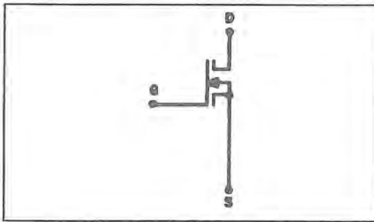
Figure 9-25. VN10LM MOSFET Without a Gate-Source Protection Diode.
