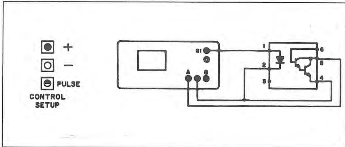
Figure 10-27. Test Circuit for a 4N31 with Pulse Generator.
