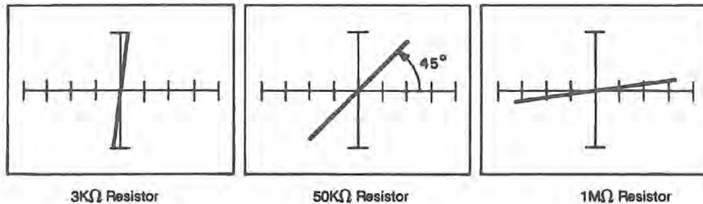
Figure 7-4. Effects of Resistance on the Rotation Angle-High Range.
