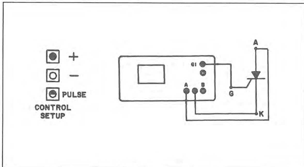
Figure 10-3. SCR Test Circuit Using Pulse Generator.
