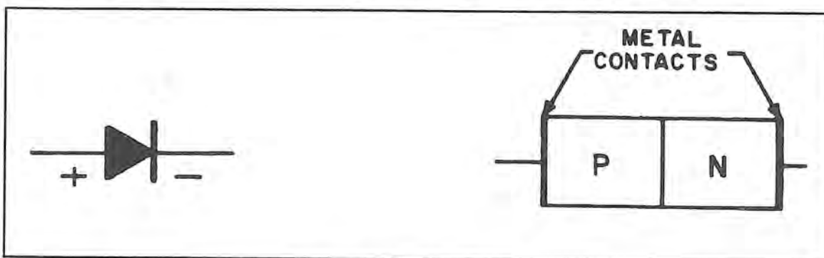
Figure 8-1. Diode Symbol.
