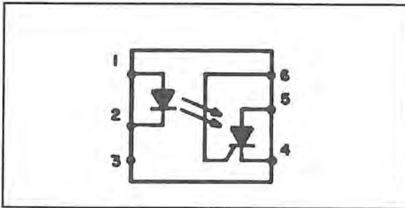
Figure 10-29. Pin Configuration of an H11C3 SCR Optocoupler.
