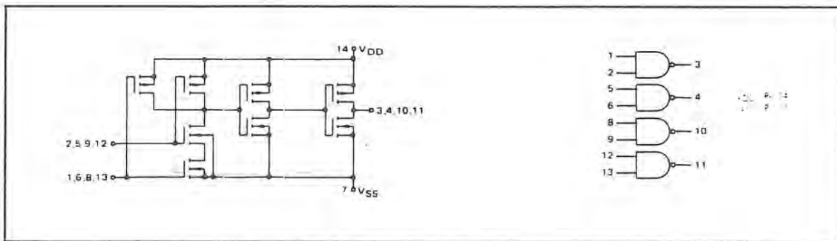
Figure 12-43. Schematic and Pin Layout of a 4011B.
