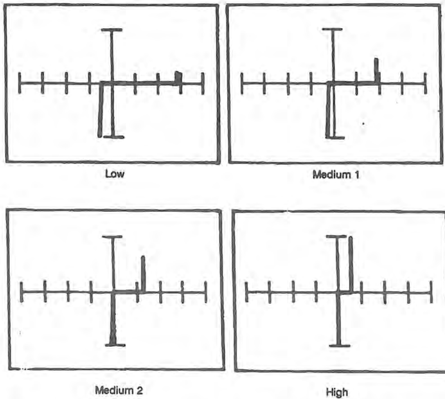
Figure 9-8. Signatures of a PNP Transistor (2N3906) at 60 Hz Base with Emitter as Common.
