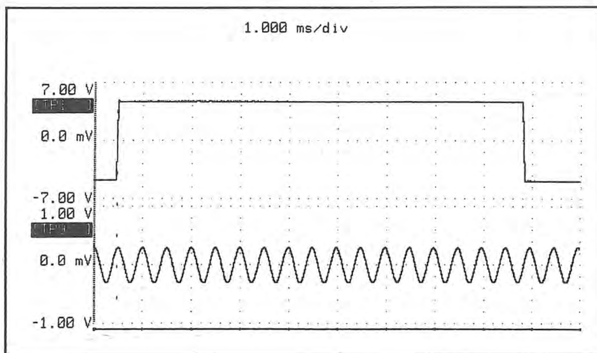
Figure 4-18. Signal PCB Waveforms: TP1 & TP9 - Settings: 2000 Hz.
