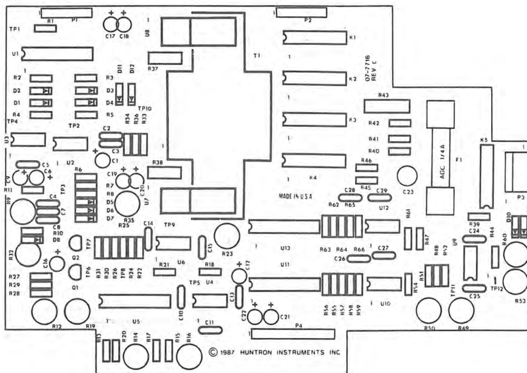
Figure 6-3. Signal PCB Component Locations
