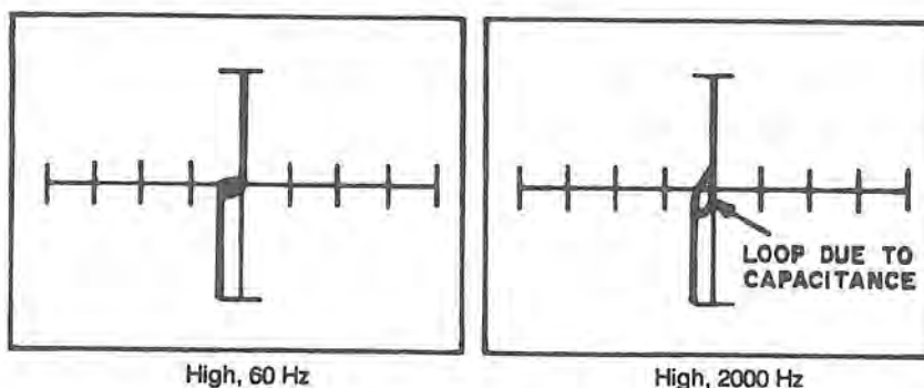
Figure 9-11. Signatures of an NPN Power Transistor (TIP50) at 60 Hz and 2000 Hz. Base with Emitter as Common.
