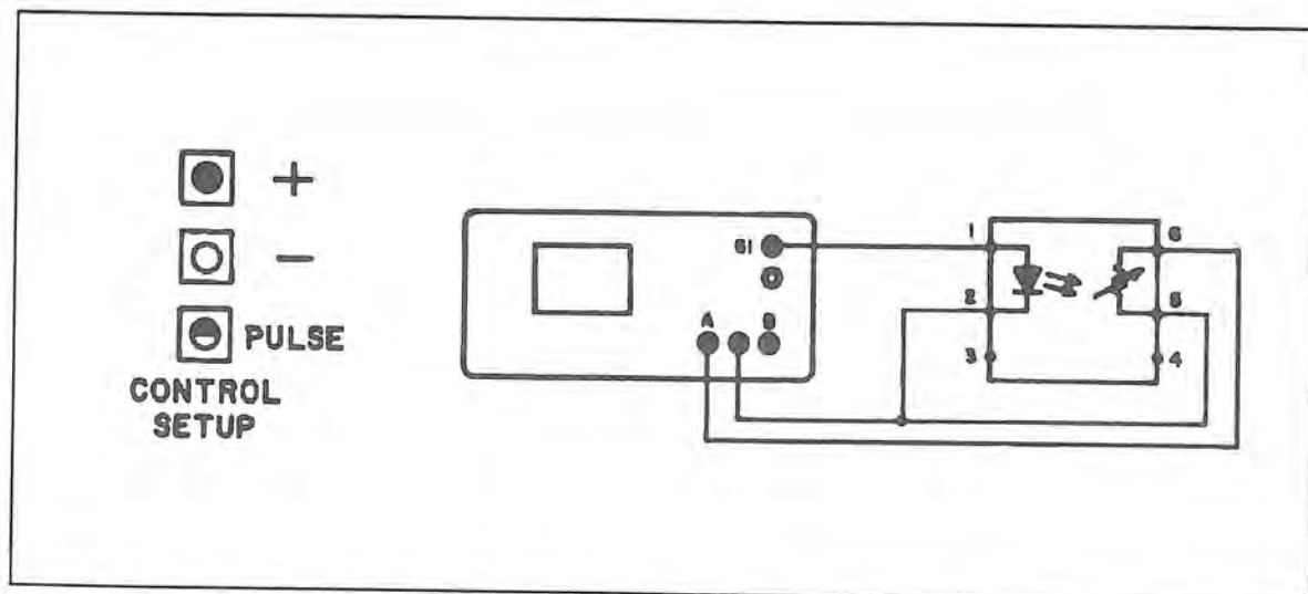
Figure 10-43. Test Circuit for a CLM51 with Pulse Generator.
