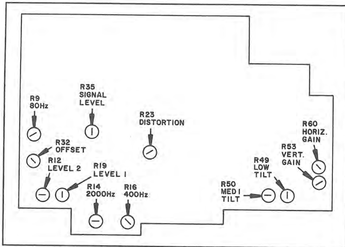
Figure 4-9. Signal PCB Adjustment Locations.
