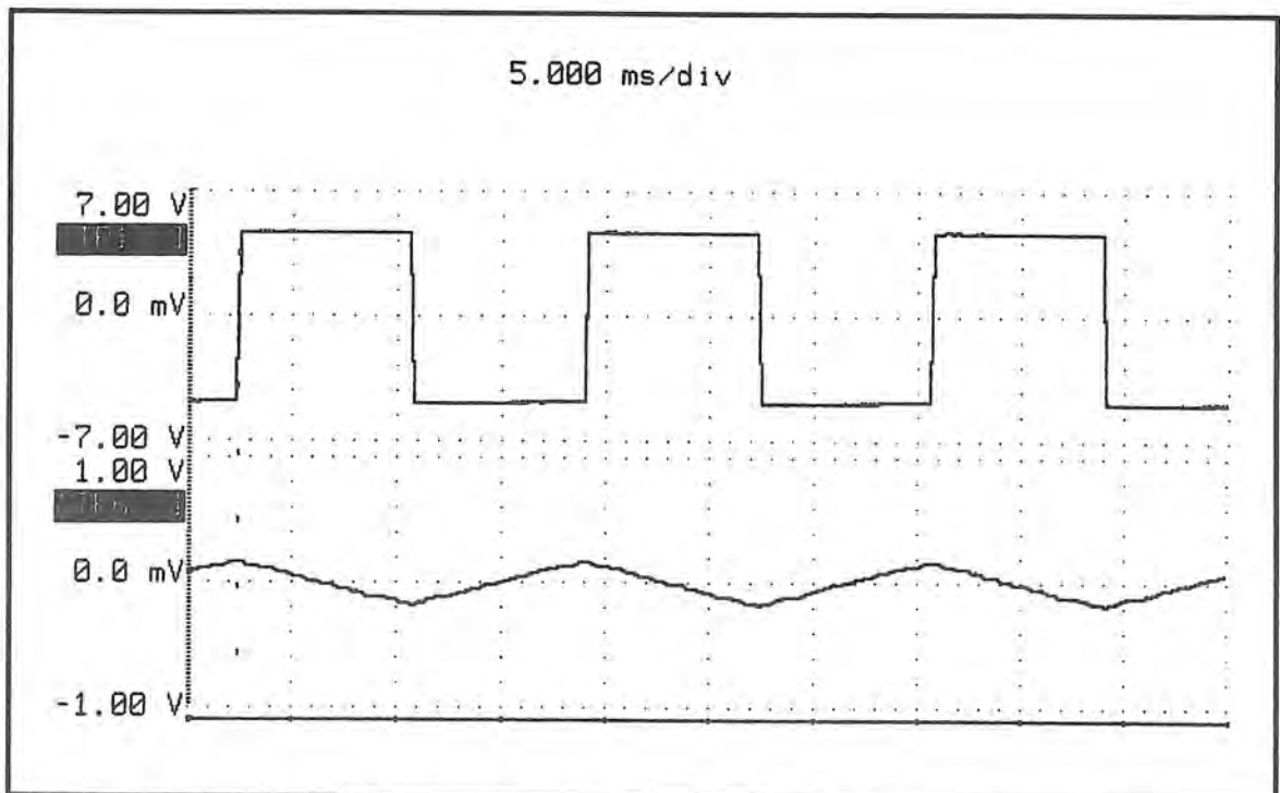
Figure 4-13. Signal PCB Waveforms: TP1 & TP6 - Settings: 50/60 Hz.
