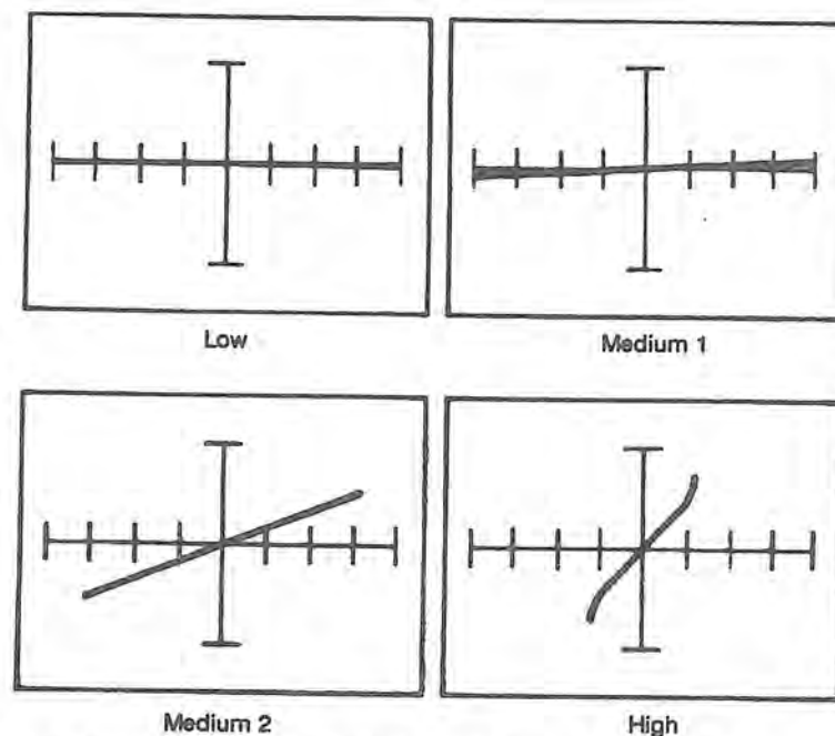
Figure 12-30. Signatures Between Pin 8 ( V_{cc} ) and Pin 1 of a Damaged LM555 Timer at 60 Hz.
