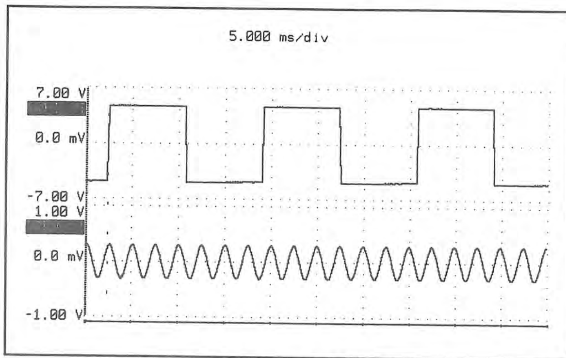
Figure 4-17. Signal PCB Waveforms: TP1 & TP9 - Settings: 400 Hz.
