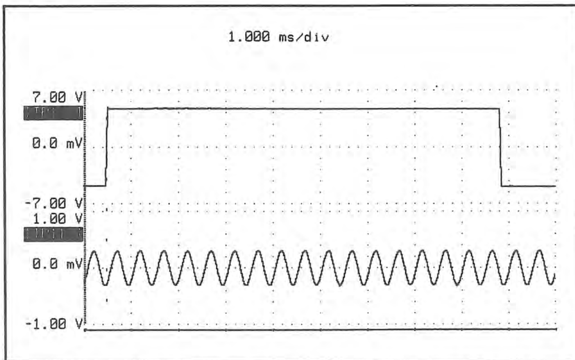
Figure 4-21. Signal PCB Waveforms: TP1 & TP11 - Settings: 2000 Hz, short circuit, LOW range.
