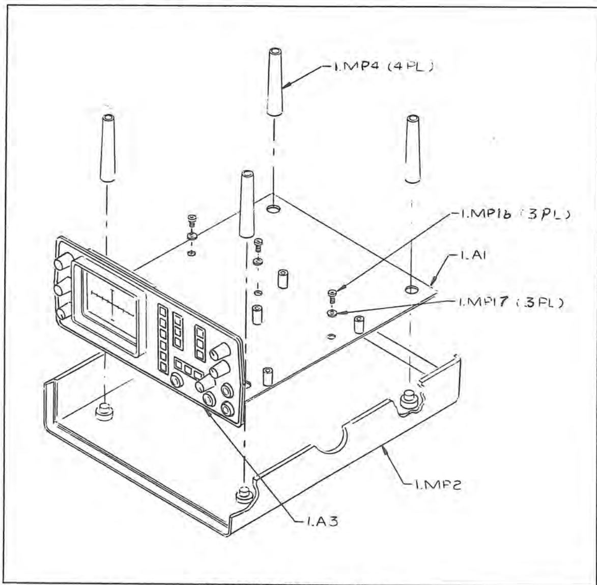
Figure 4-5. Main PCB Assembly Removal.
