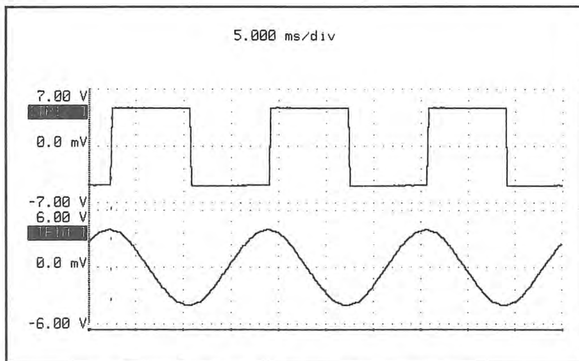
Figure 4-19. Signal PCB Waveforms: TP1 & TP10 - Settings: 50/60 Hz, LOW range.
