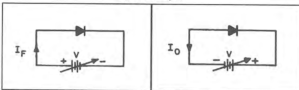
Figure 8-2. P-N Junction Biased in the Forward Direction.
