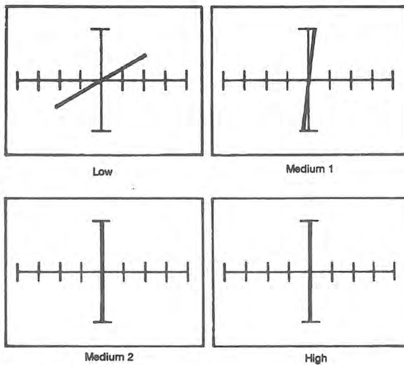
Figure 12-10. Signatures Between Pin 8 (V+) and Pin 4 (V-) of a Defective LM1458 at 60 Hz.
