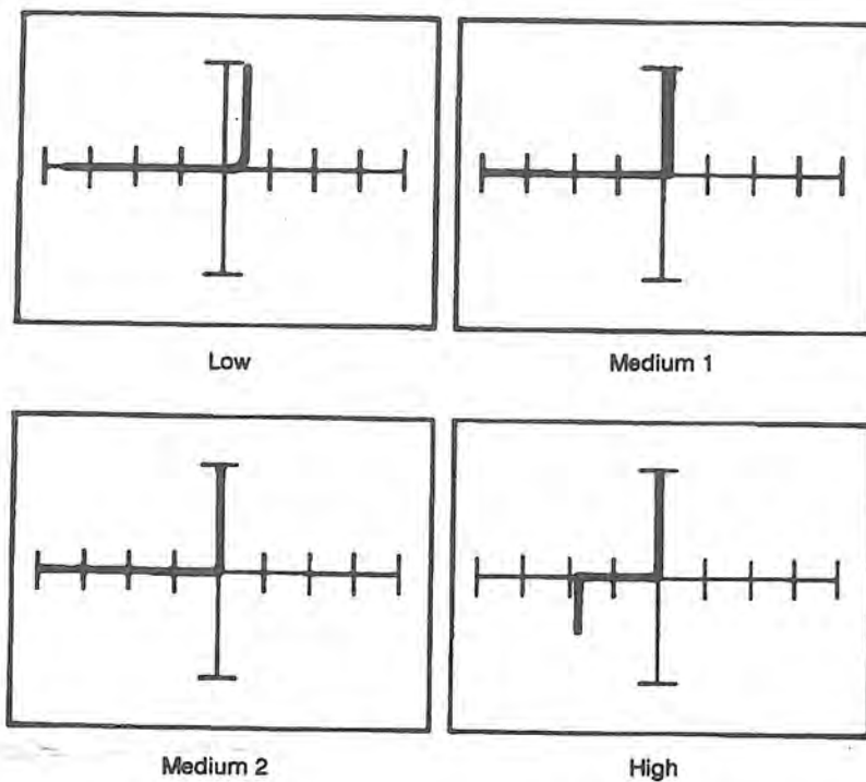
Figure 10-2. Signatures of a C103 SCR at 60 Hz. Gate with Cathode as Common.
