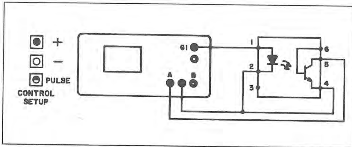
Figure 10-20. Optocoupler Test Connections Using Pulse Generator.
