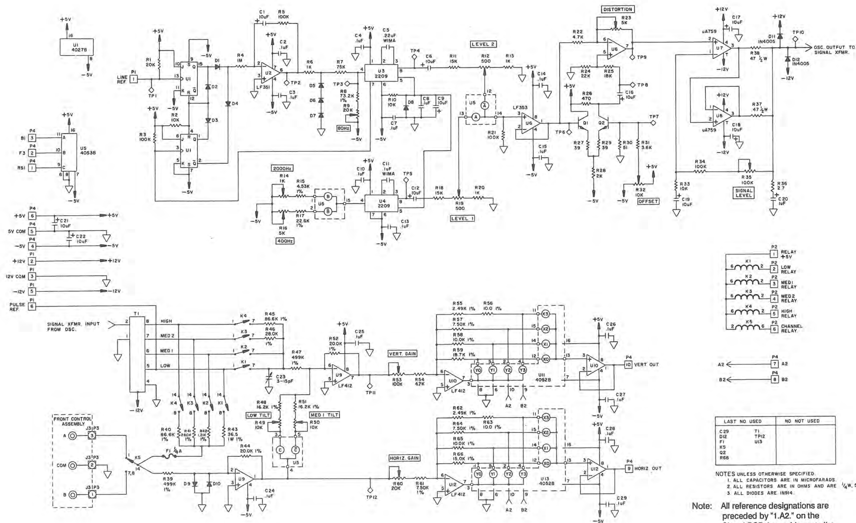
Figure 6-4. Signal PCB Schematics
