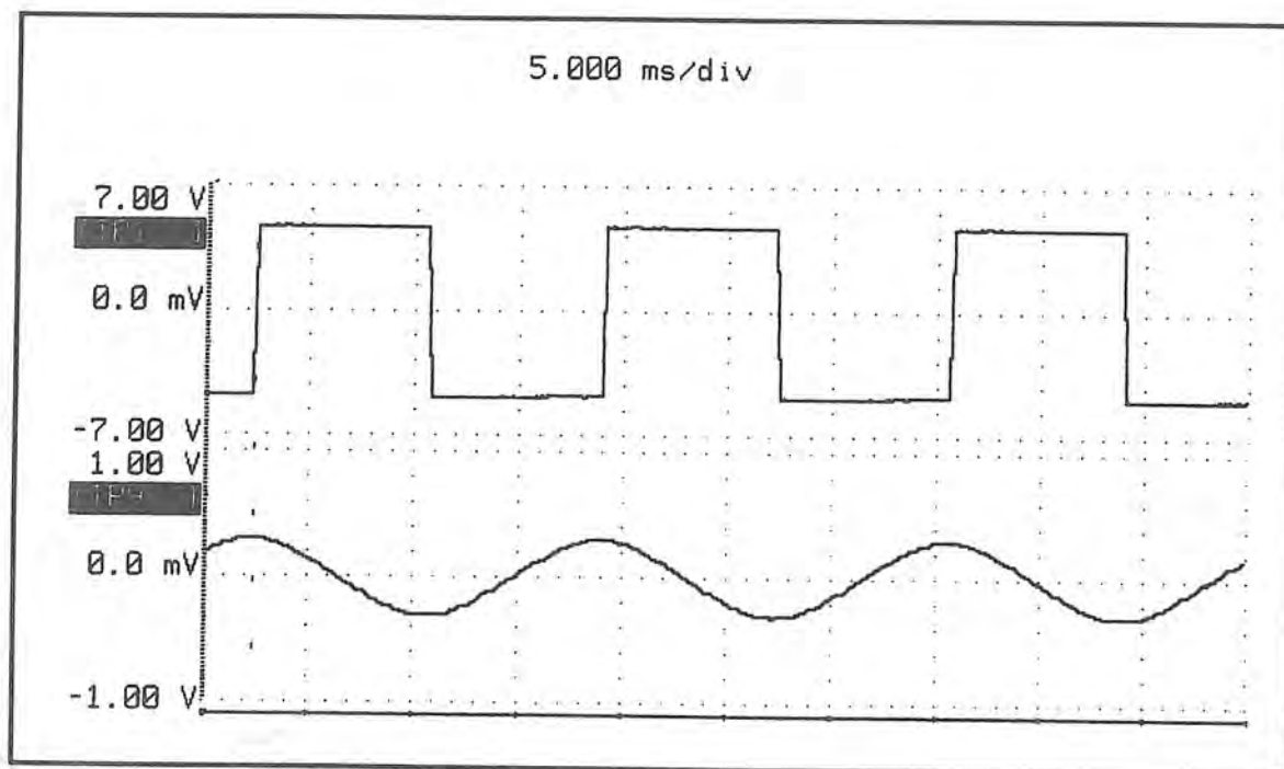
Figure 4-16. Signal PCB Waveforms: TP1 & TP9 - Settings: 50/60 Hz.
