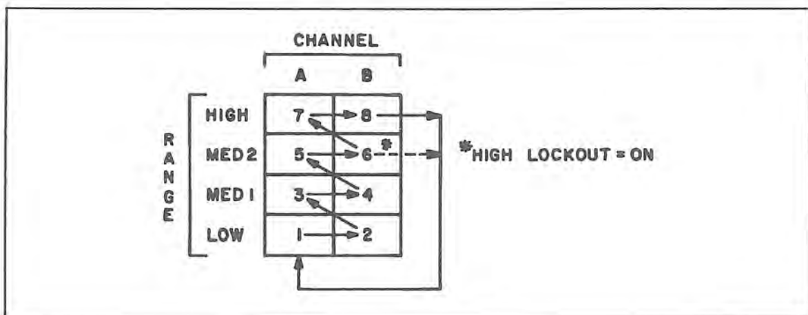
Figure 2-5. Auto/Alternate Sequence.
