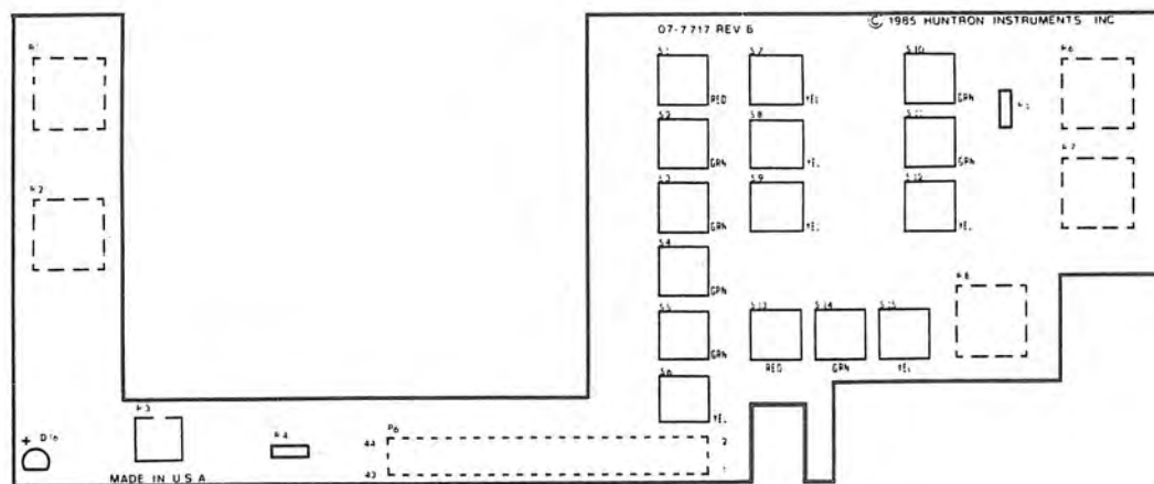
Figure 6-5. Control PCB Component Locations
