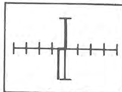
Figure 9-15. Signature Comparison of a Darlington Transistor (TIP112) and a Regular Transistor (TIP29) at 60 Hz. Base with Emitter as Common.
