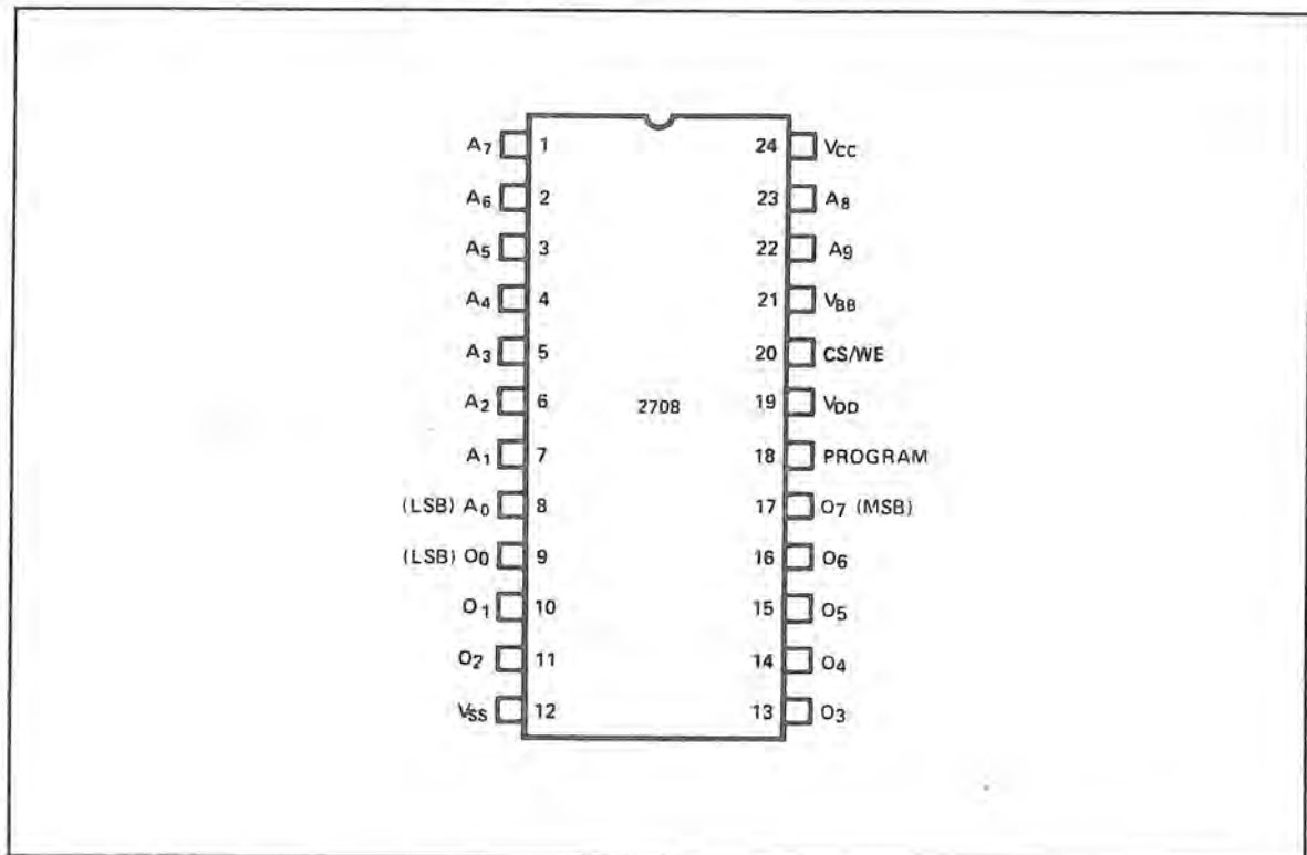
Figure 12-57. Pin Layout of a 2708JL.
