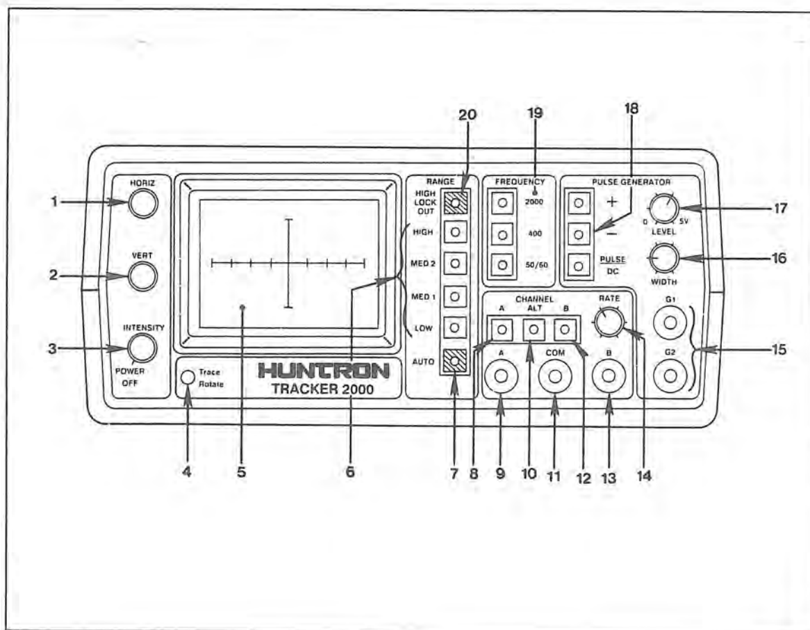
Figure 2-1. Front Panel.
