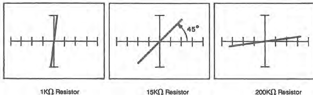
Figure 7-3. Effect of Resistance on the Rotation Angle - Medium 2 Range.
