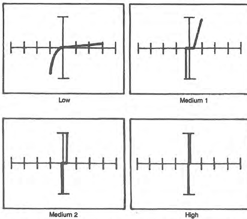
Figure 12-32. Signatures Between the V_{cc} Pin and the Ground Pin of a 7410 at 60 Hz.
