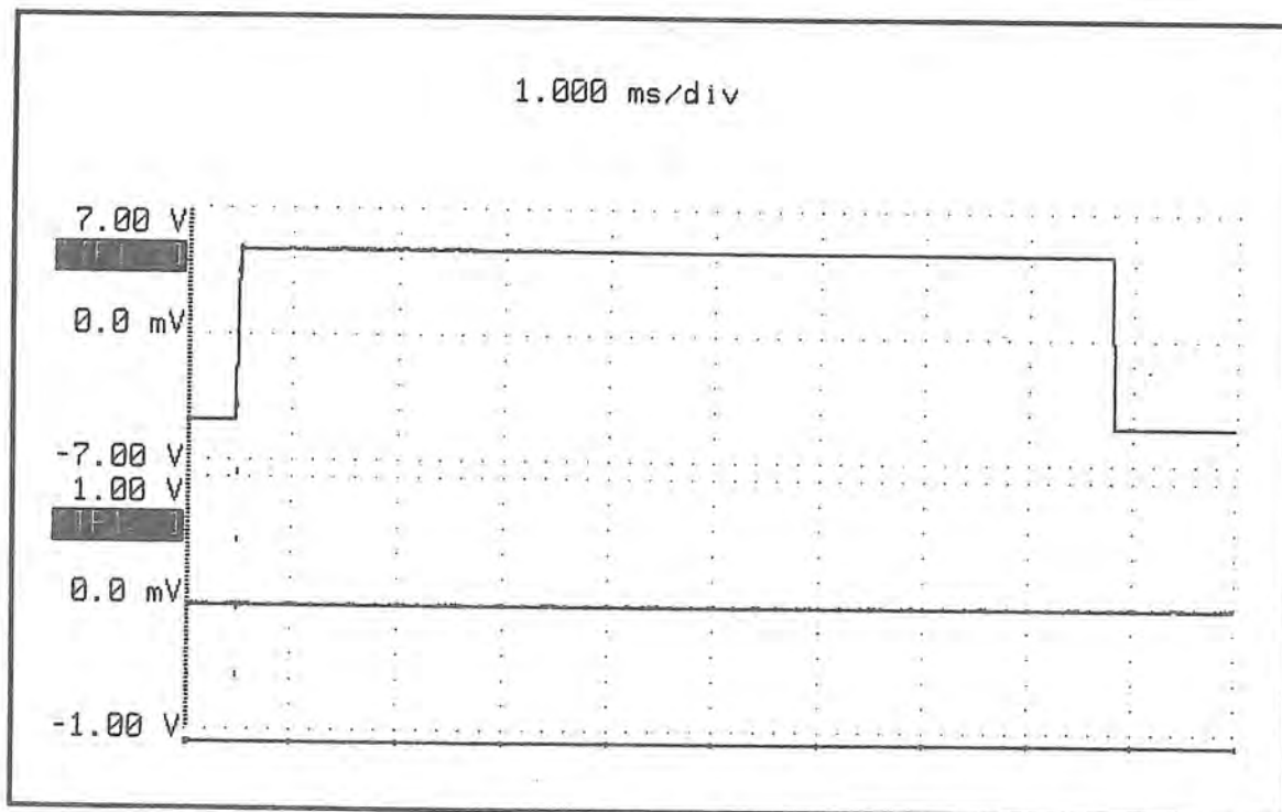
Figure 4-23. Signal PCB Waveforms: TP1 & TP12 - Settings: 2000 Hz, short circuit, LOW range.
