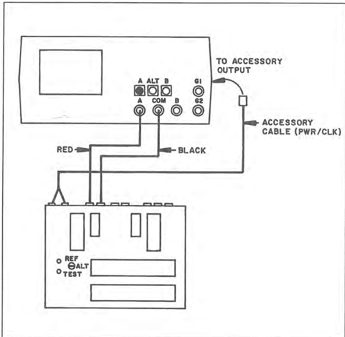
Figure 2-8. 2000/Switcher Interconnection.
