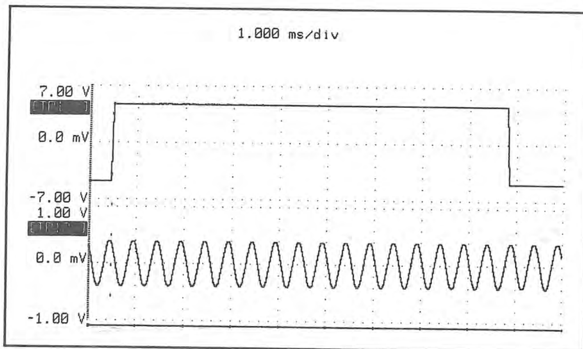
Figure 4-22. Signal PCB Waveforms: TP1 & TP12 - Settings: 2000 Hz, open circuit, LOW range.
