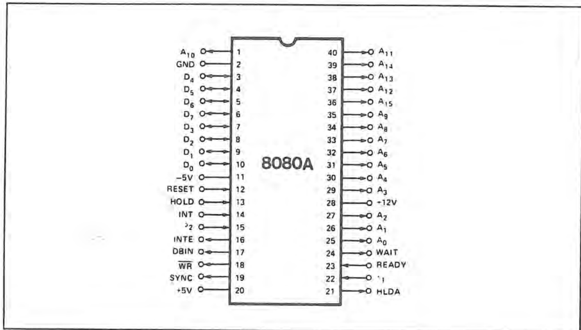
Figure 12-78. Pin Layout of an 8080A
