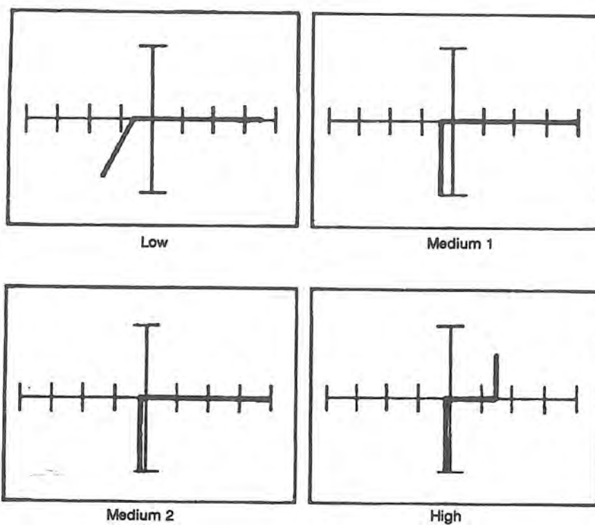
Figure 12-71. Signatures Between the V_{LC} Pin and the V^- Pin of a DAC0800L at 60 Hz.
