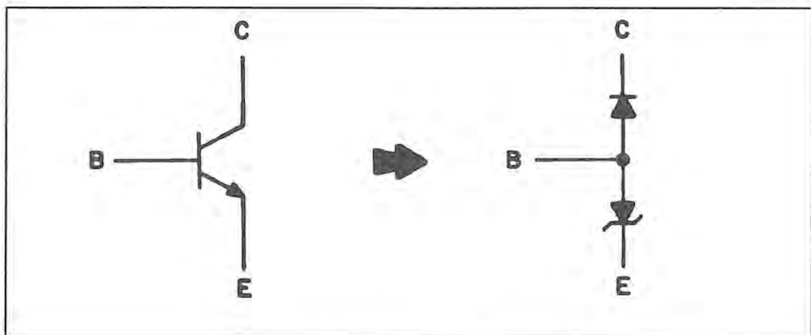
Figure 9-3. Equivalent Circuit of an NPN Transistor.
