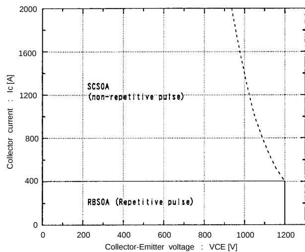
Reversed biased safe operating area +V_{GE}=15V , -V_{GE} \leq 15V , T_J \leq 125^\circ C , R_G \geq 4.7ohm
