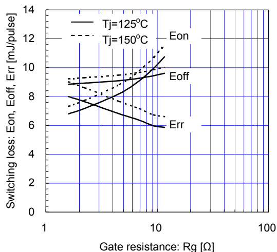
Switching loss vs. Gate resistance (typ.) Vcc=600V, Ic=100A, VGE=±15V, Tj=125, 150°C
