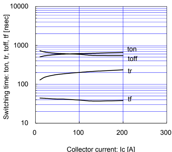
Switching time vs. Collector current (typ.) Vcc=600V, VGE=±15V, Rg=1.6Ω, Tj=125°C
