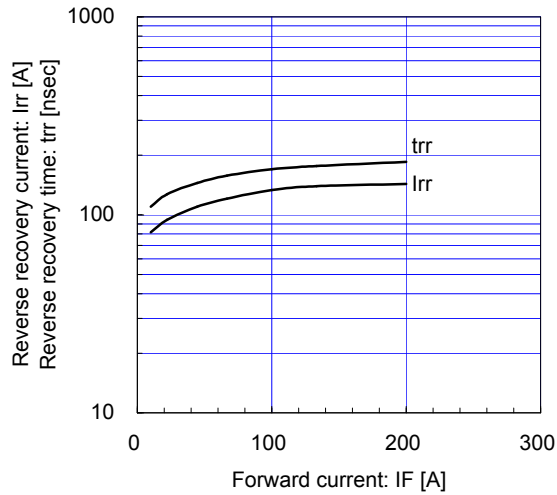
Reverse Recovery Characteristics (typ.) Vcc=600V, VGE=±15V, Rg=1.6Ω, Tj=150°C
