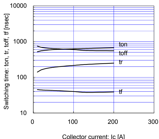
Switching time vs. Collector current (typ.) Vcc=600V, VGE=±15V, Rg=1.6Ω, Tj=150°C
