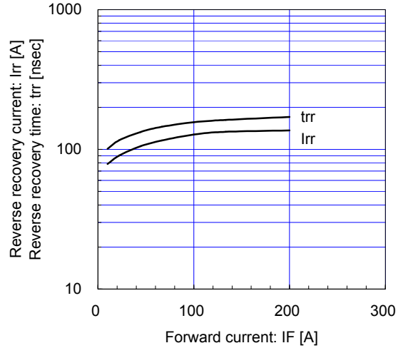
Reverse Recovery Characteristics (typ.) Vcc=600V, VGE=±15V, Rg=1.6Ω, Tj=125°C
