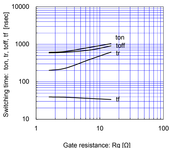
Switching time vs. Gate resistance (typ.) Vcc=600V, Ic=100A, VGE=±15V, Tj=125°C
