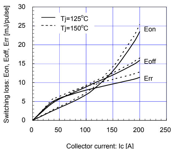
Switching loss vs. Collector current (typ.) Vcc=600V, VGE=±15V, Rg=1.6Ω, Tj=125, 150°C
