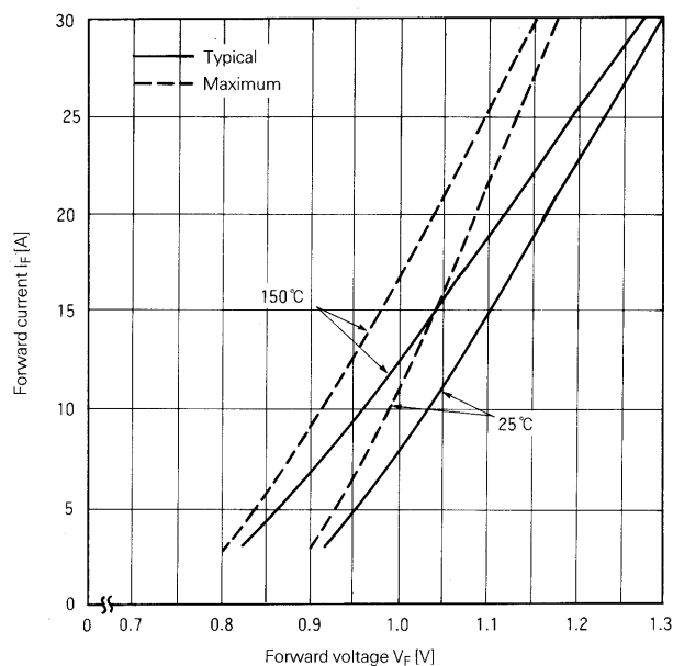
Forward Characteristics
