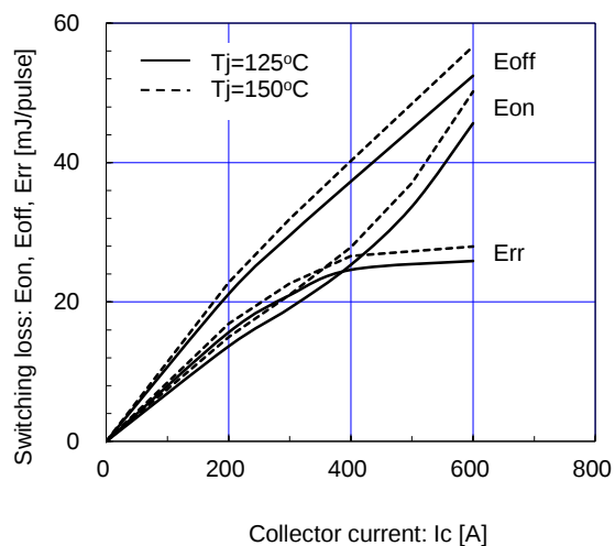
Switching loss vs. Collector current (typ.) V_{CC}=600V , V_{GE}=\pm 15V , R_g=1.8\Omega , T_j=125^\circ C
