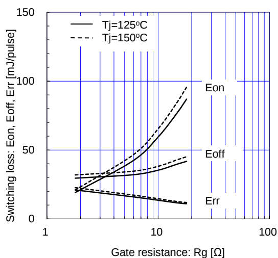
Switching loss vs. Gate resistance (typ.) V_{CC}=600V , I_c=300A , V_{GE}=\pm 15V , T_j=125^\circ C
