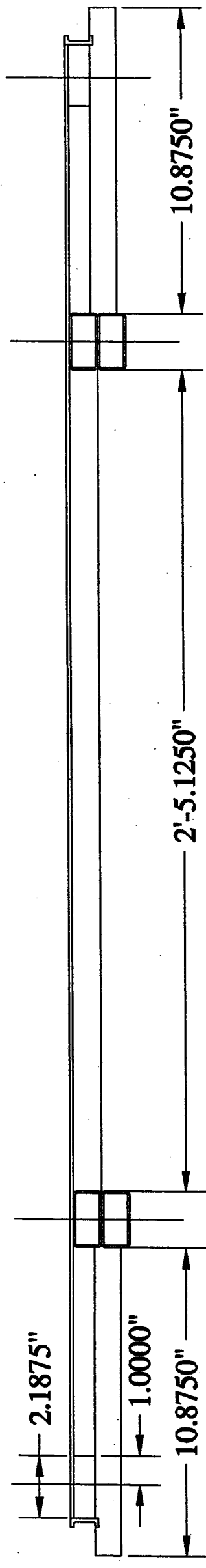
BOTTOM VIEW
