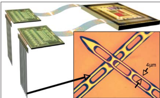
New WIMS ERC probe designs being driven by the need for long-term tissue-compatible interfaces.
