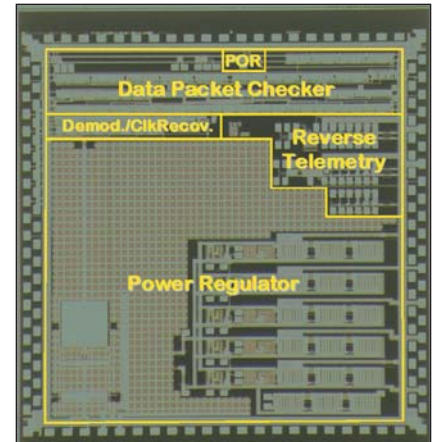
Six components of the chip.
