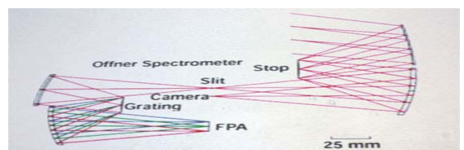
Optical path of the Fore Optics in the Moon Mineralogy Mapper
