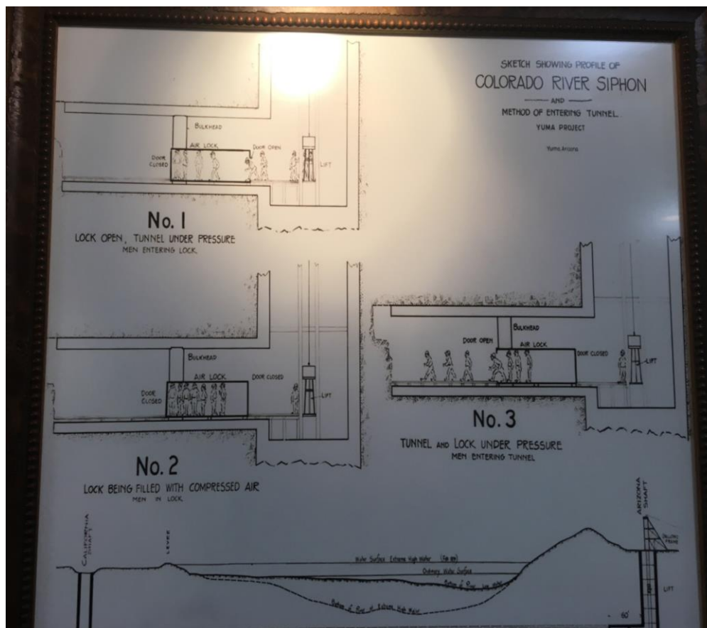
Colorado River Siphon Drawings (Photo courtesy of Jack Moody)
