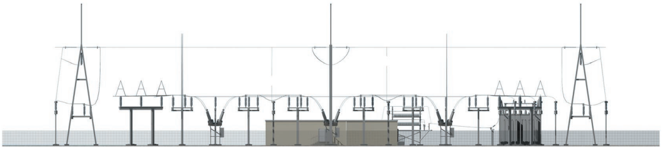
North Elevation
