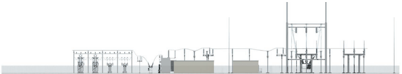
East Elevation
