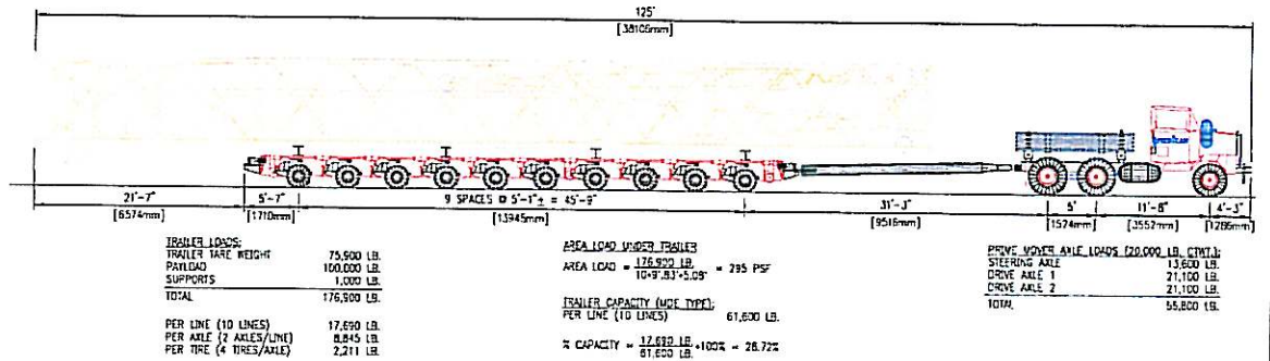
BOOM HAULING DIAGRAM
