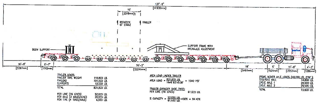
CRANE HAULING DIAGRAM
