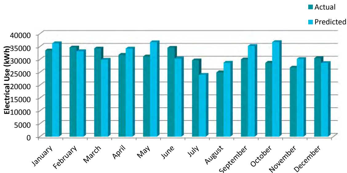
Figure 4.2-19: Pleasantdale Elementary Electricity Usage
