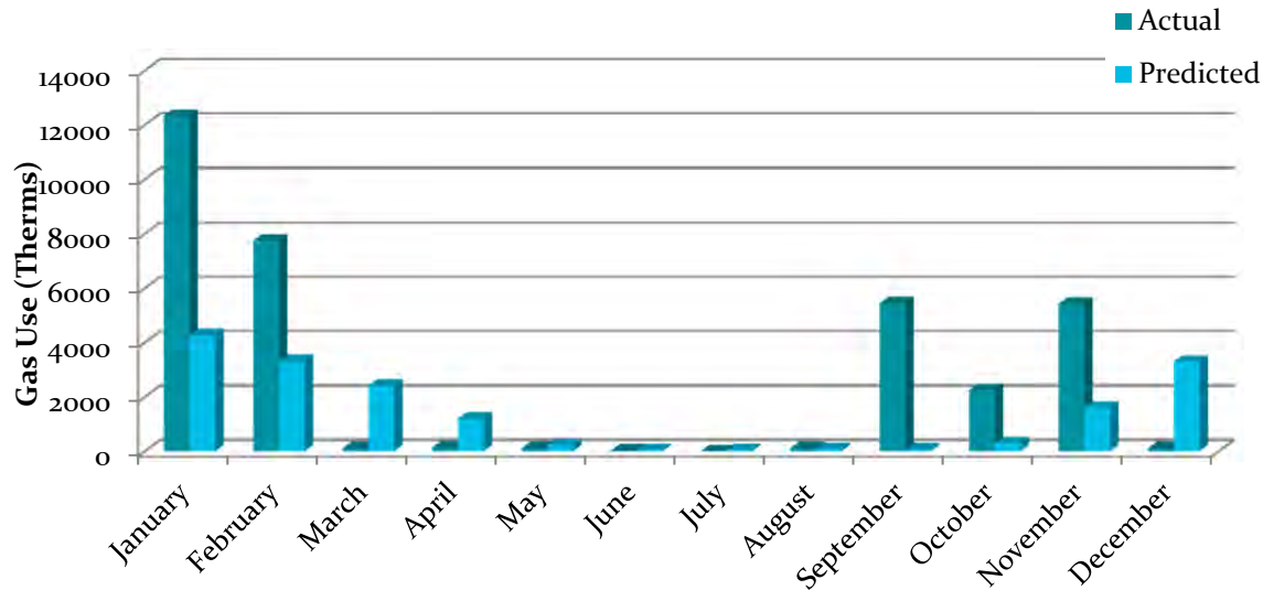
Figure 4.2-24: Redwood Elementary Natural Gas Usage
