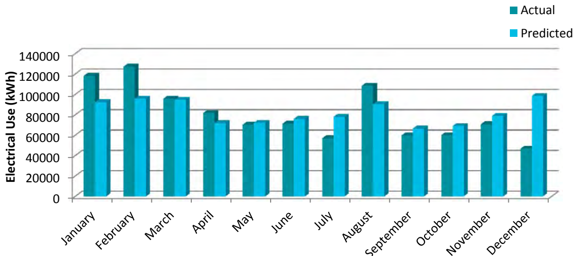
Figure 4.2-25: Roosevelt Middle School Electricity Usage
