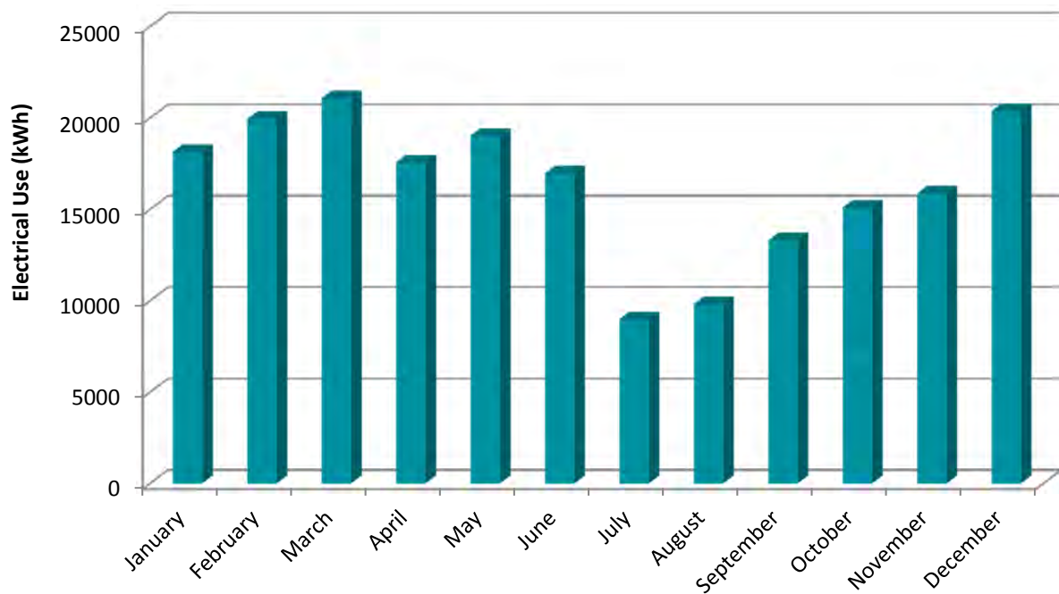
Figure 3.2-19: St. Cloud Elementary School Electricity Usage
