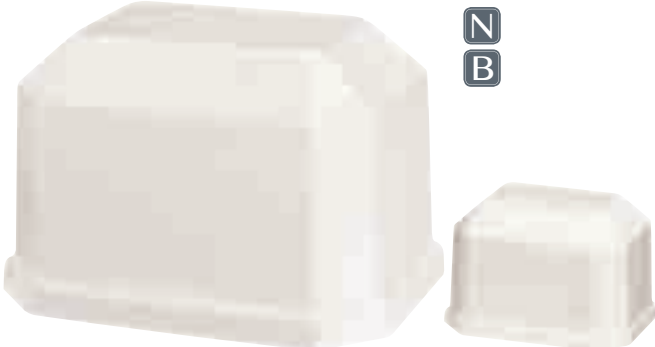
3WM420 3WM420KS WHITE MARBLE WHITE MARBLE KEEPSAKE 7" H x 10.625" W x 8" D 2.625" H x 4" W x 3" D CULTURED MARBLE CULTURED MARBLE Volume: 200ci Volume: 6ci Access: Bottom Access: Bottom
