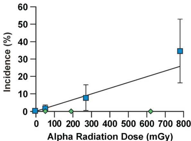
Figure 1. Lung Cancer Incidence in Wistar Rats: after inhalation exposure to the alpha radiation source ^{239}\text{PuO}_2 (squares) or ^{239}\text{PuO}_2 labeled with a yttrium-169 gamma-emitting tag (diamonds). The added gamma exposure (1-2 mGy) prevented alpha-radiation-induced lung cancers, presumably via gamma-ray ANP. None of the 1877 animals receiving gamma rays (diamonds) in addition to their alpha radiation exposure developed lung cancer for the indicated dose range. The data are from Sanders, 21 and for the indicated dose range a total of 3793 animals were used. Error bars are 95% CI, assuming a binomial distribution of cancer cases.
