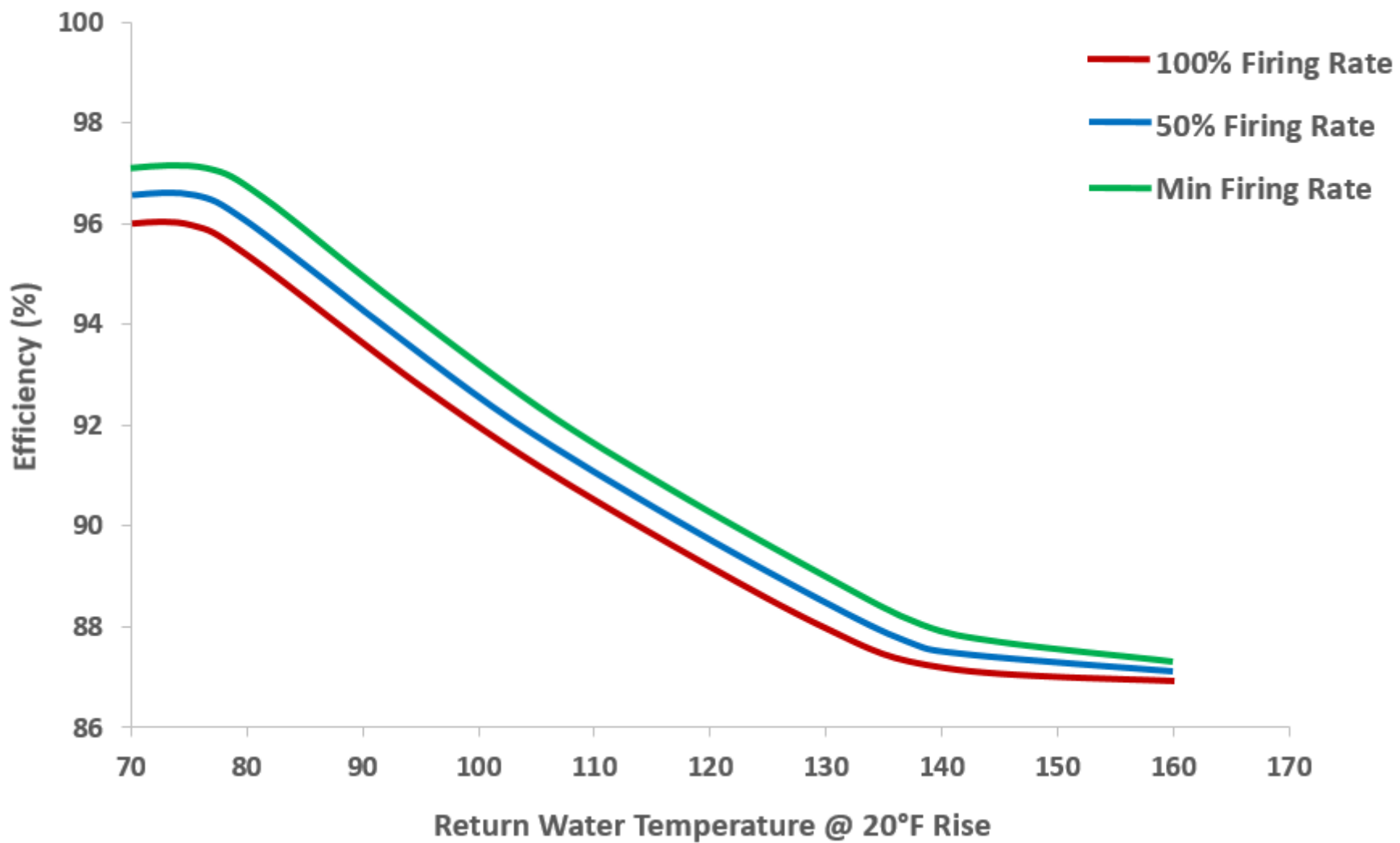
XFIIRE Efficiency Curves
