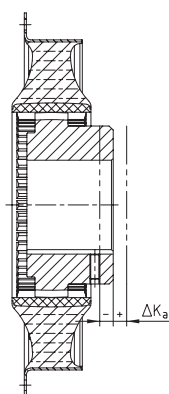
Axial displacement
