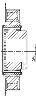
Radial displacement
