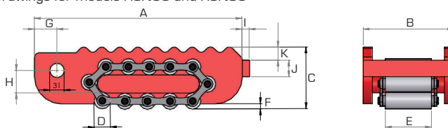
Drawings for models RSN60 and RSN80
