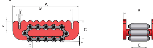
Drawings for models RSN60 and RSN80
