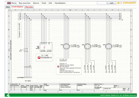
User-defined visualisation
