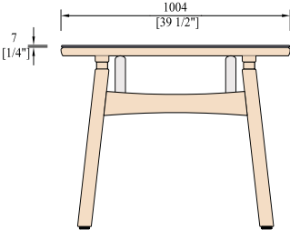
Technical drawing of the Monterey dining table – Teak with ceramic table top
