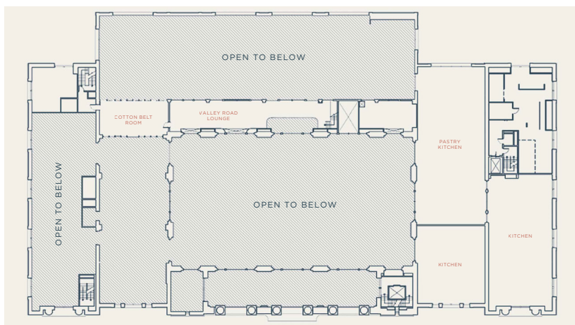
UPPER MEZZANINE LEVEL
