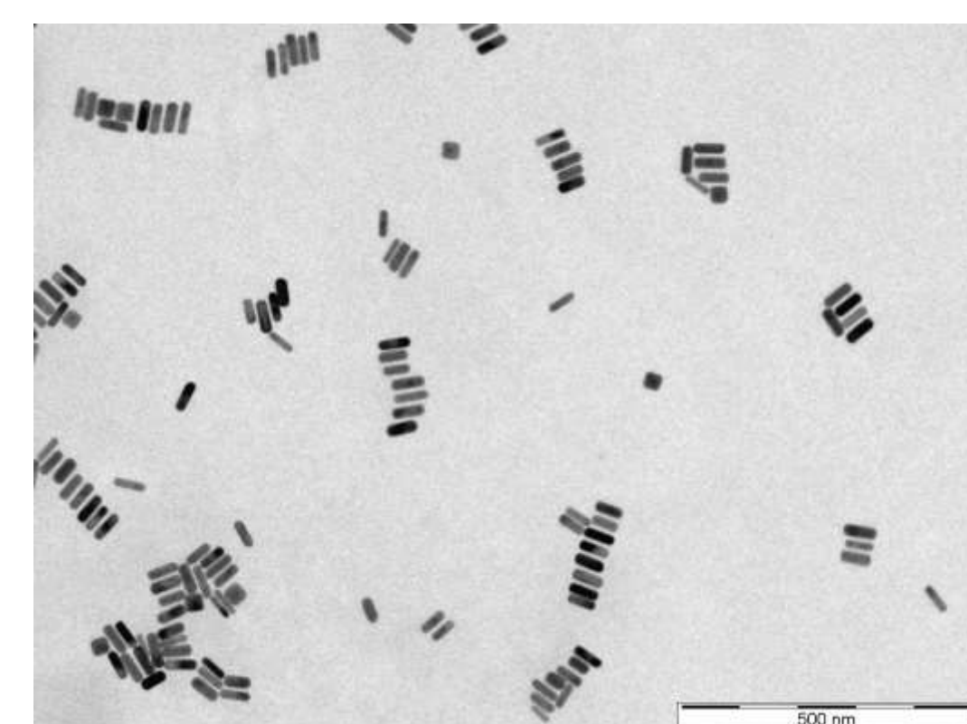
TEM image of the synthesized gold nanorods. The rods had an aspect ratio of ~3 (45 nm long/15 nm diameter)
