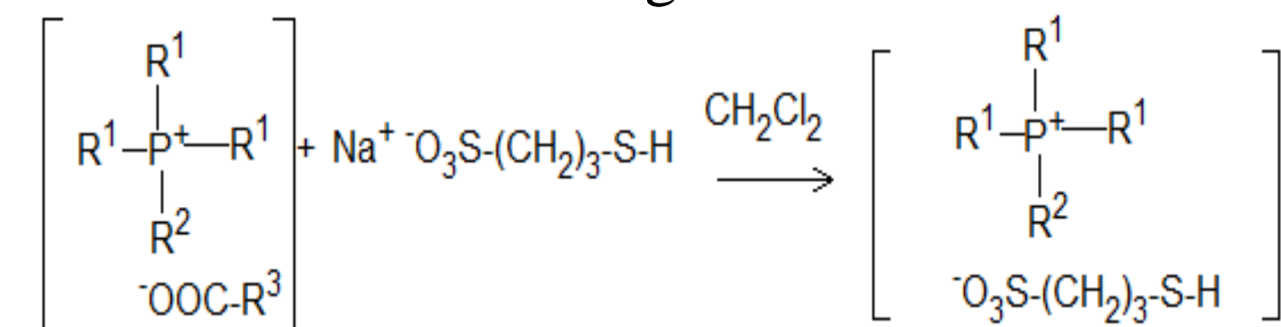
The corona (right) is prepared by simple ion exchange of a phosphonium salt with sodium mercapto-propanesulfonate and then filtration in dichloromethane.
