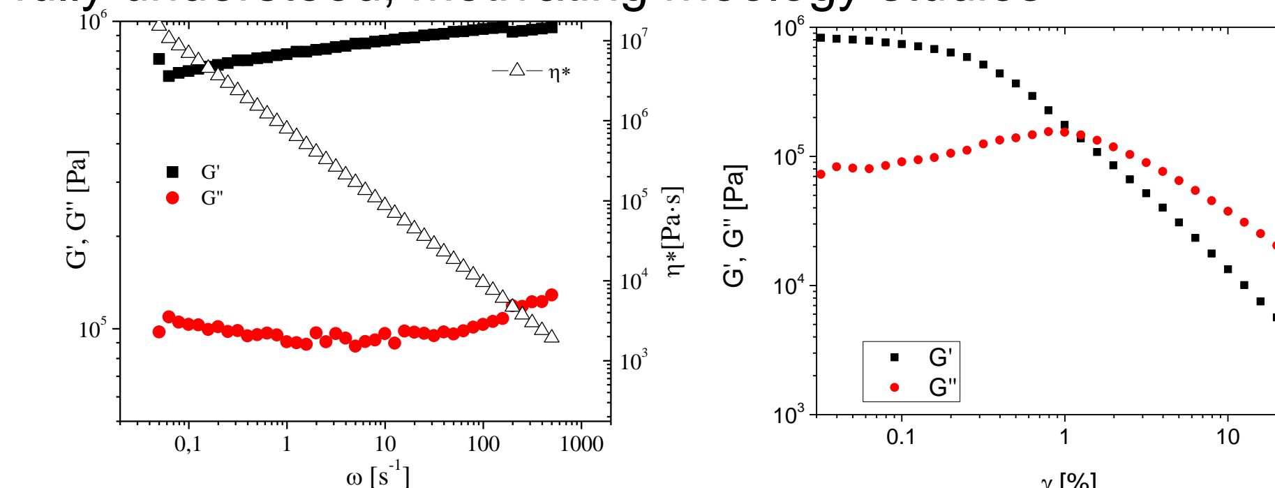
Left: Oscillatory amplitude sweep at ω = 50 s -1 showing the characteristic soft glass peak in G' at crossover.
