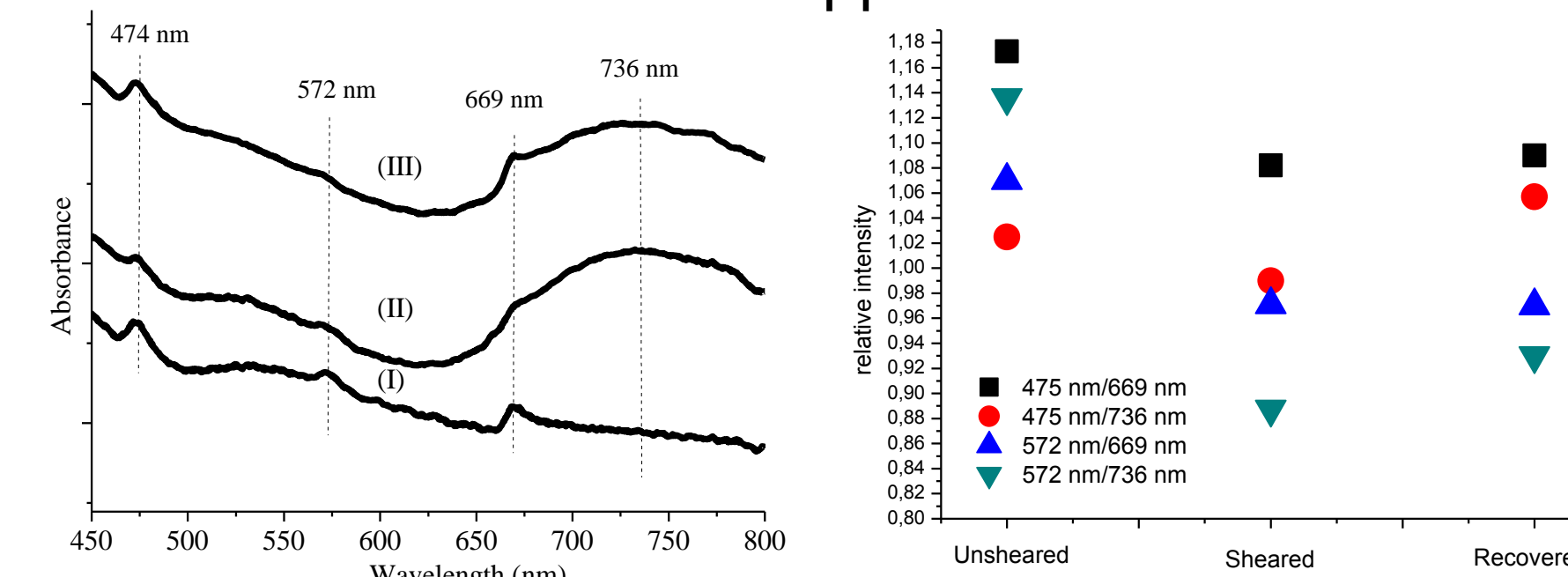
Left: The solid-state spectra of the gels in the initial state (I), after shearing in one direction (II) and sheared back in the opposite direction (III)
