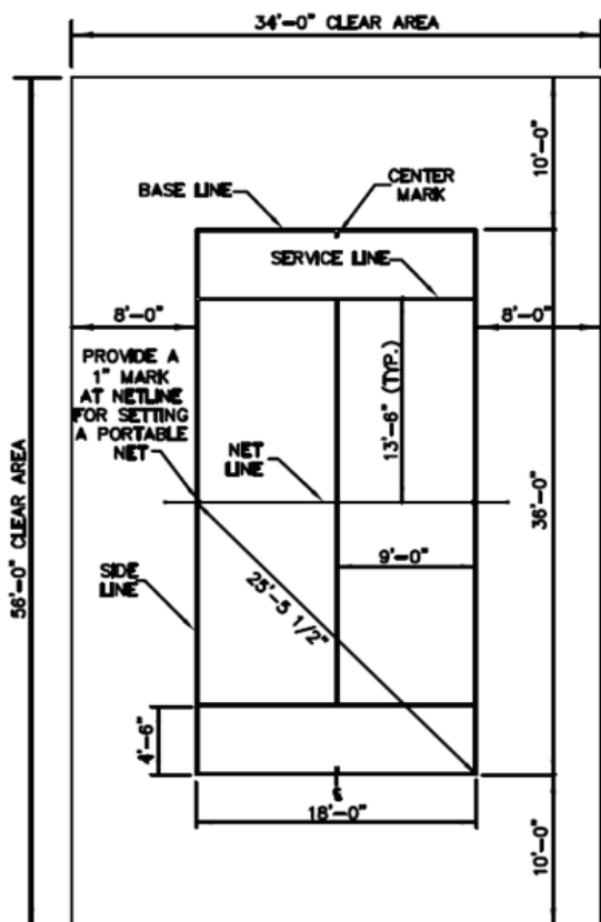
SINGLE COURT LAYOUT
