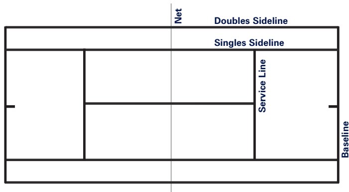
Full-Size Court
