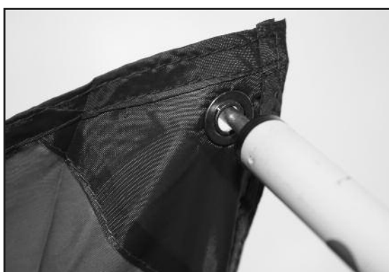
STEP 13 - Insert the pin of the assembled awning pole into the grommet of the awning as shown.
