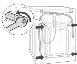
Unpacking and removing shipping bolts
