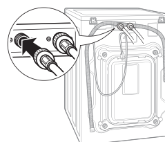
Connecting the water line
