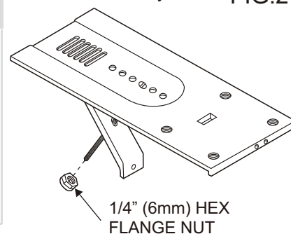
Platform Assembly FIG.21
