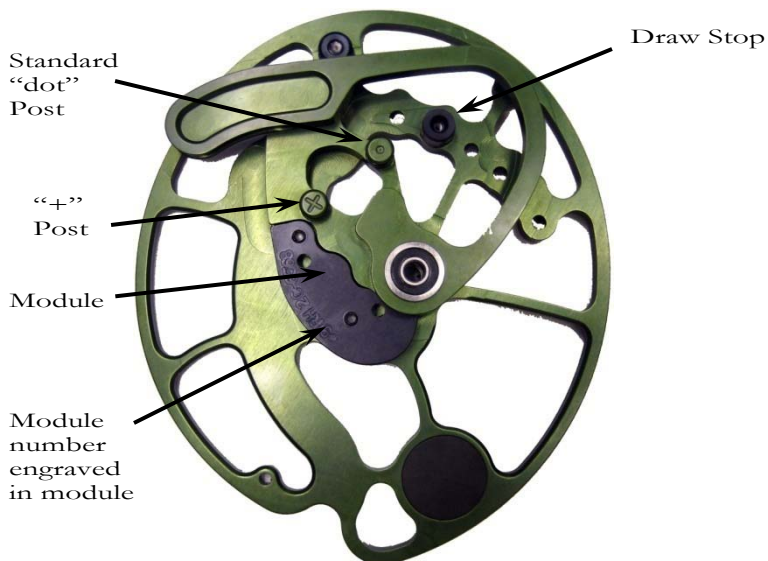
Back View
