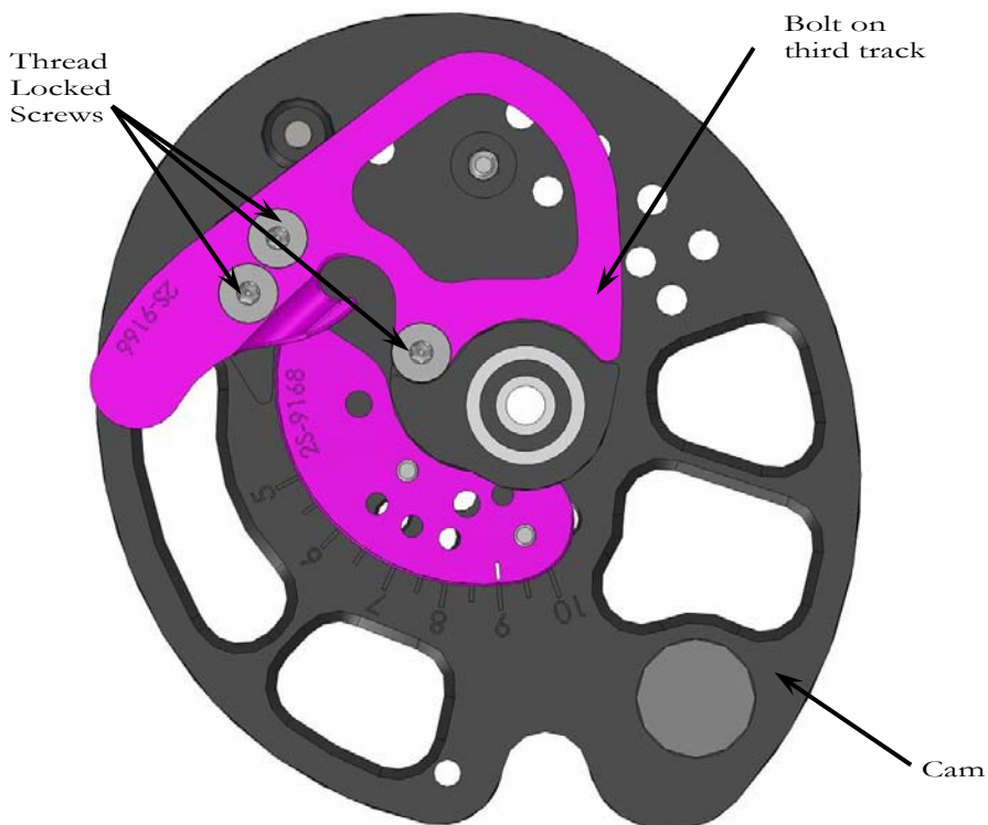
Siren Rotating Module Cam Back View
