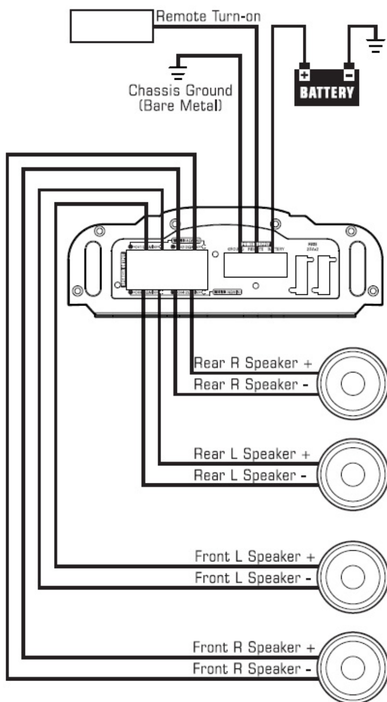
Figure 3 Connections for power and speakers
