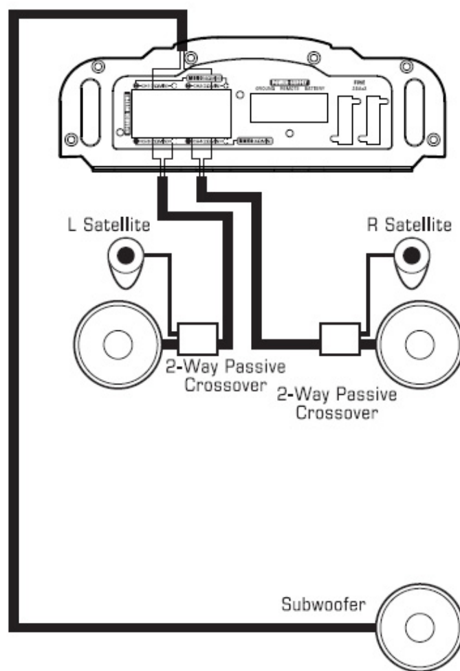
Figure 6 The AP-1504 can also be used to drive a pair of stereo satellites for the front and a single mono subwoofer for the rear. Note the filter settings.
