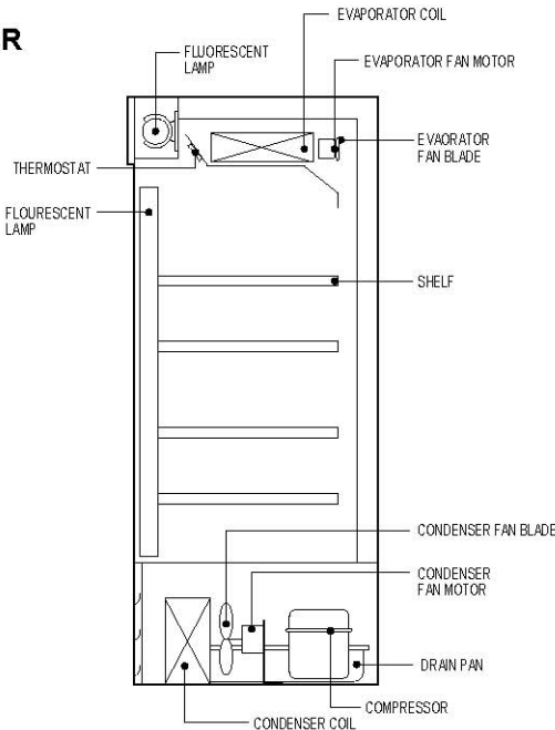
< SIDE >
