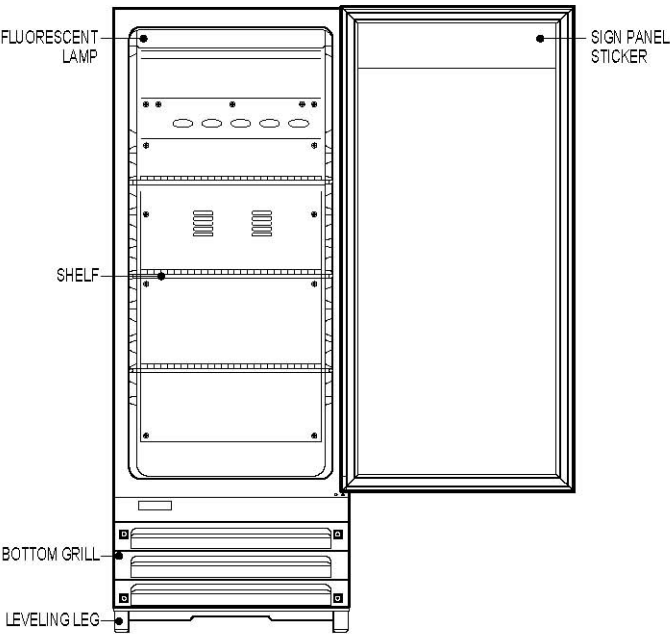
< FRONT >
