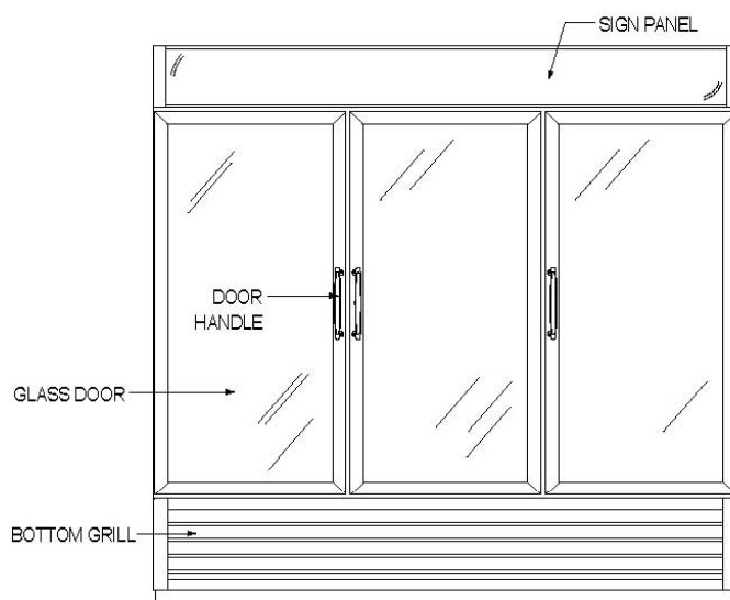
< FRONT >
