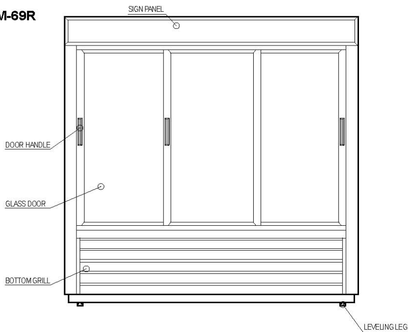
< FRONT >
