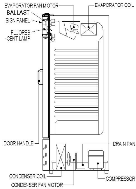
< SIDE >
