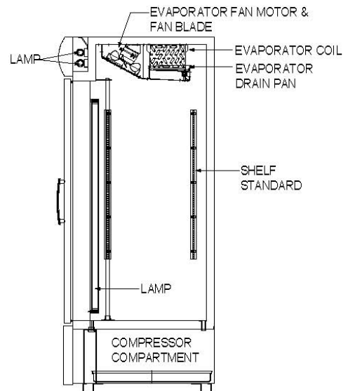
< SIDE >
