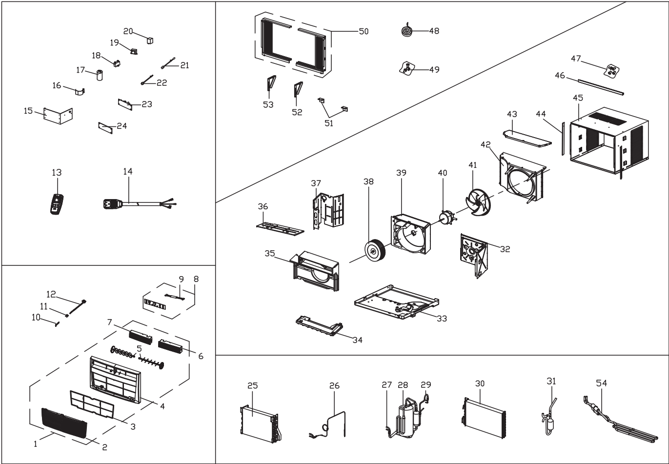
FRA256ST210-1 Parts
