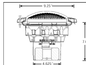
Cross Section of Jandy Pool Light
