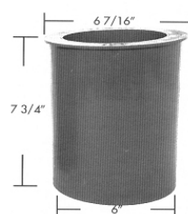
B-38 American 850012 Weir
