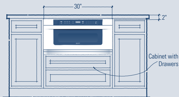
STANDARD INSTALLATION WITH DRAWERS BELOW
