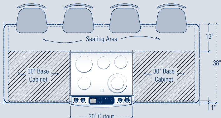
ISLAND COOKING AND PREPPING AREA WITH SEATING
